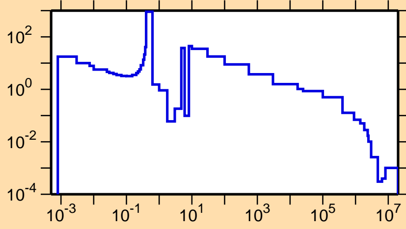
\sigma vs. E for ^{232}\text{Fr}(n,\gamma)
