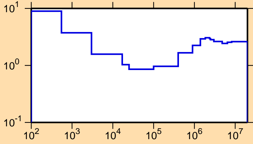
\sigma vs. E for ^{232}\text{Fr}(n,\text{nonel.})
