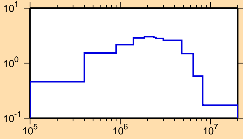
\sigma vs. E for ^{232}\text{Fr}(n,n\text{cont.})
