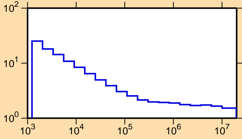
\sigma vs. E for ^{63}\text{Ga}(n,\text{nonel.})
