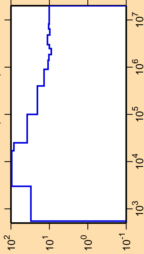
\Delta\sigma/\sigma vs. E for ^{63}\text{Ga}(n,\text{nonel.})
