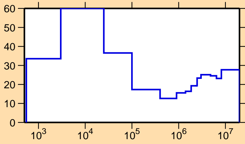
\Delta\sigma/\sigma vs. E for ^{63}\text{Ga}(n,p)
