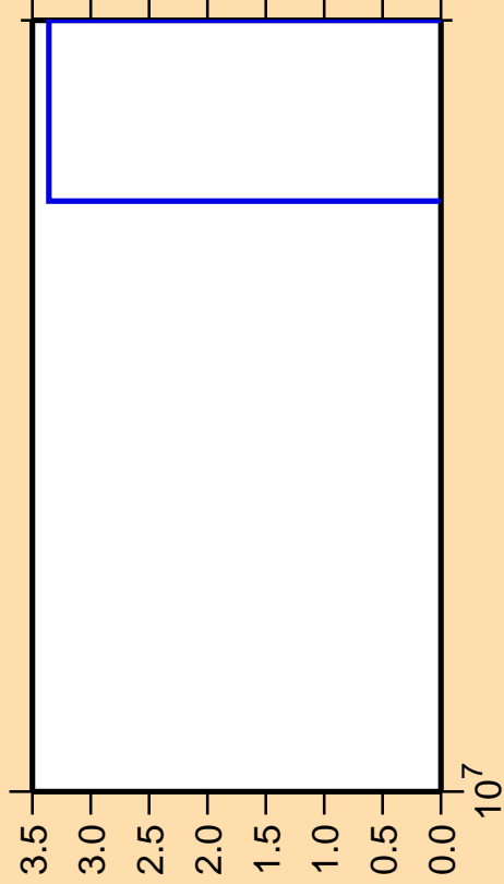
\Delta\sigma/\sigma vs. E for ^{64}\text{Ga}(n,nt)
