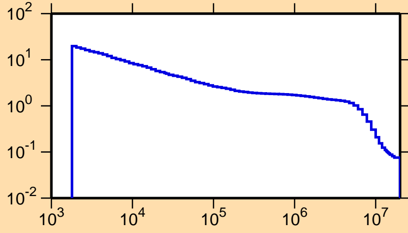
\sigma vs. E for ^{64}\text{Ga}(n,p)
