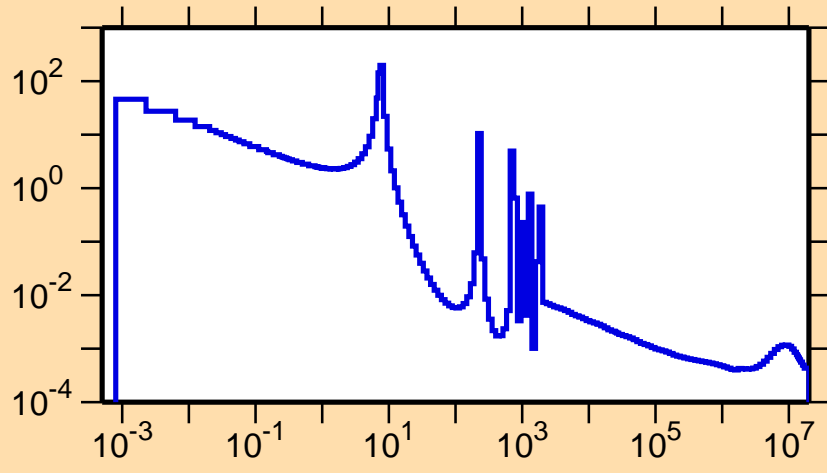
\sigma vs. E for ^{64}\text{Ga}(n,\gamma)
