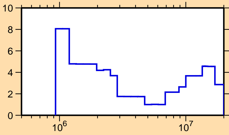
\Delta\sigma/\sigma vs. E for ^{64}\text{Ga}(n,\text{tot.})
