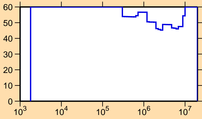
\Delta\sigma/\sigma vs. E for ^{64}\text{Ga}(n,\gamma)
