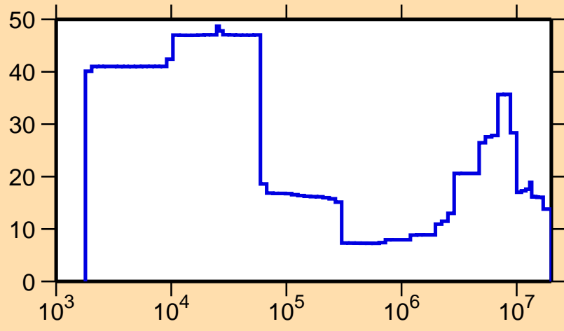
\Delta\sigma/\sigma vs. E for ^{64}\text{Ga}(n,p)
