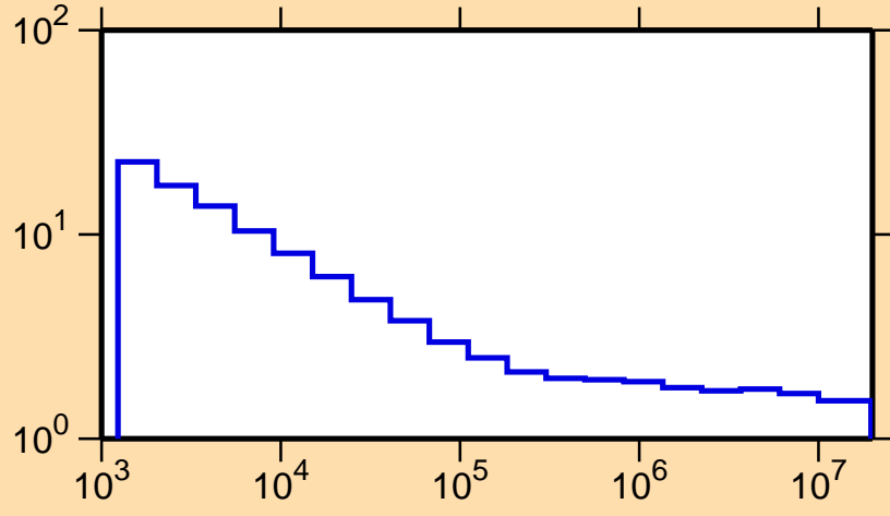
\sigma vs. E for ^{64}\text{Ga}(n,\text{nonel.})
