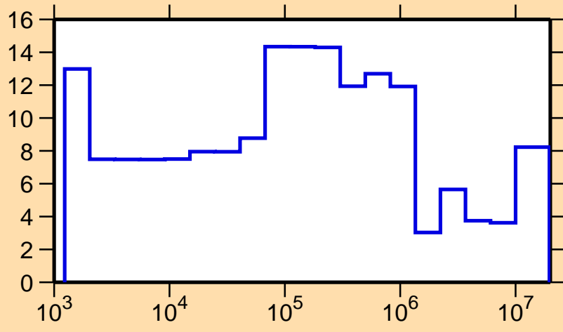
\Delta\sigma/\sigma vs. E for ^{64}\text{Ga}(n,el.)
