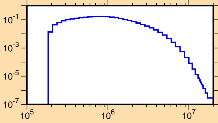
\sigma vs. E for ^{65}\text{Ga}(n,n_2)
