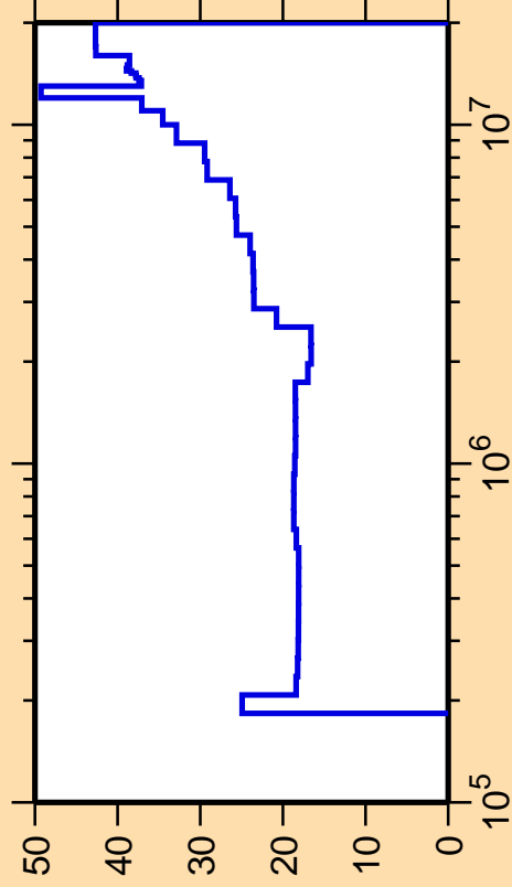
\Delta\sigma/\sigma vs. E for ^{65}\text{Ga}(n,n_2)
