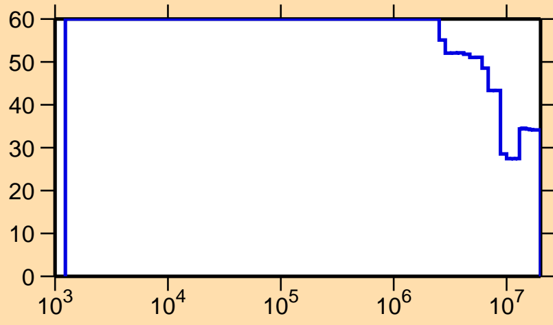
\Delta\sigma/\sigma vs. E for ^{65}\text{Ga}(n,\gamma)
