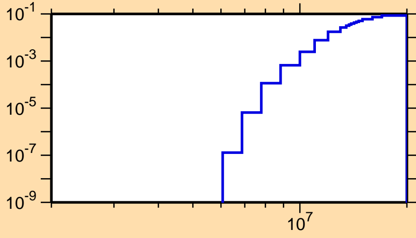
\sigma vs. E for ^{65}\text{Ga}(n,n\alpha)
