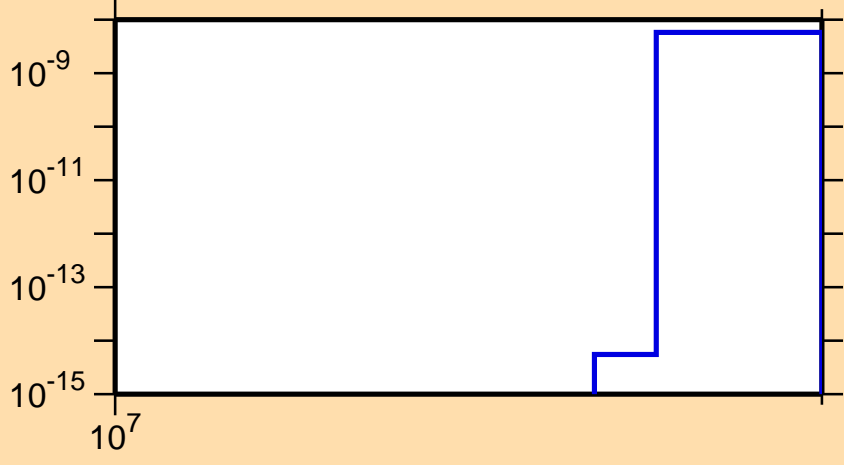
\sigma vs. E for ^{65}\text{Ga}(n,nt)
