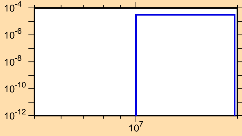
\sigma vs. E for ^{65}\text{Ga} (mt 45)
