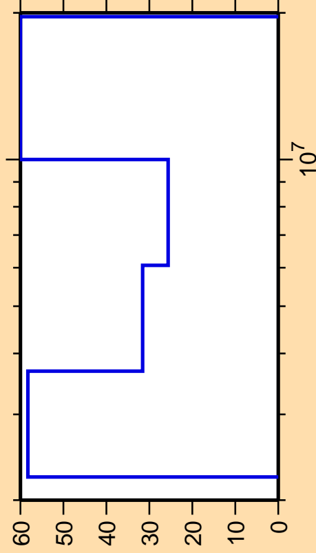
\Delta\sigma/\sigma vs. E for ^{65}\text{Ga}(n,d)
