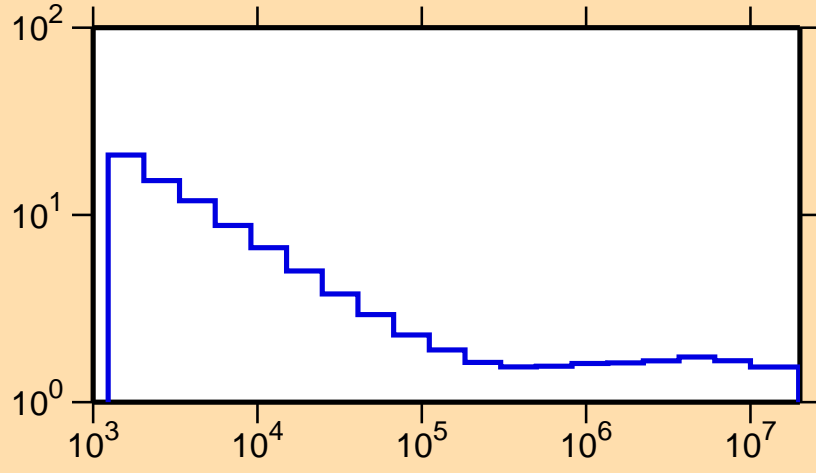
\sigma vs. E for ^{65}\text{Ga}(n,\text{nonel.})
