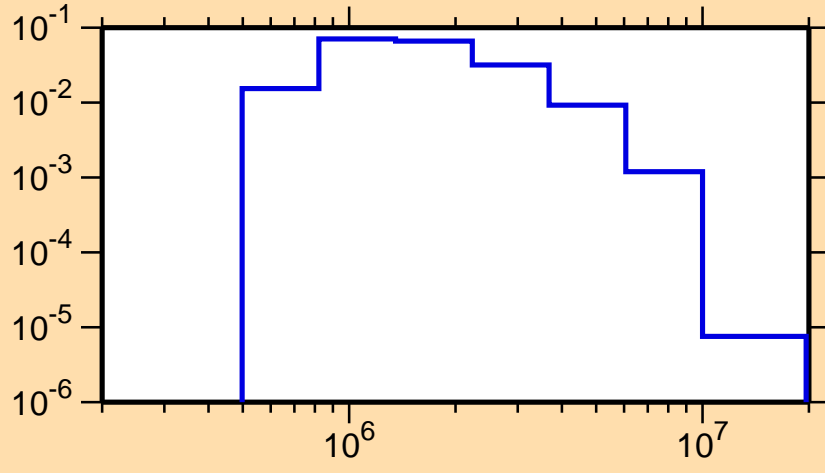
\sigma vs. E for ^{65}\text{Ga}(n,n_3)
