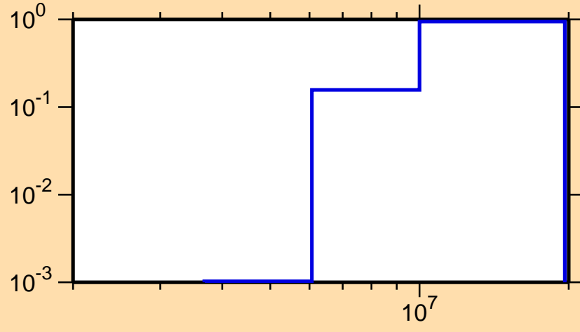
\sigma vs. E for ^{65}\text{Ga}(n,np)
