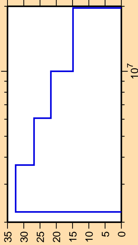
\Delta\sigma/\sigma vs. E for ^{65}\text{Ga}(n,n\text{cont.})
