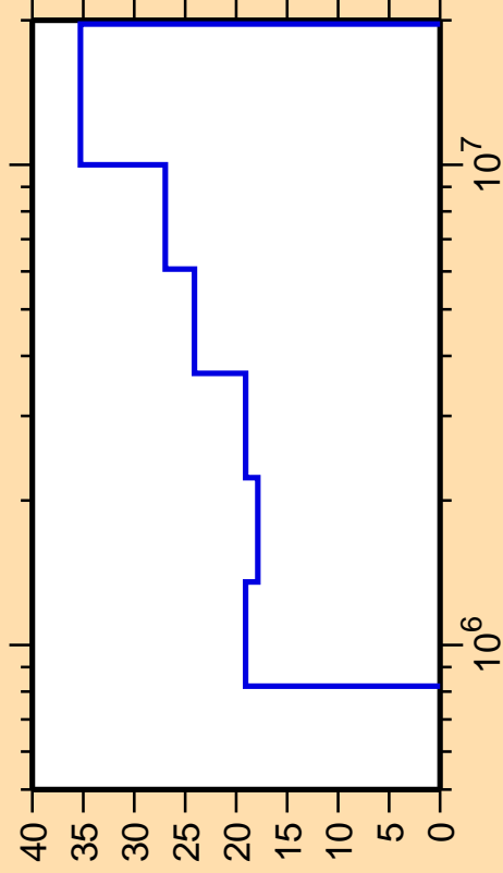
\Delta\sigma/\sigma vs. E for ^{65}\text{Ga}(n,n_4)
