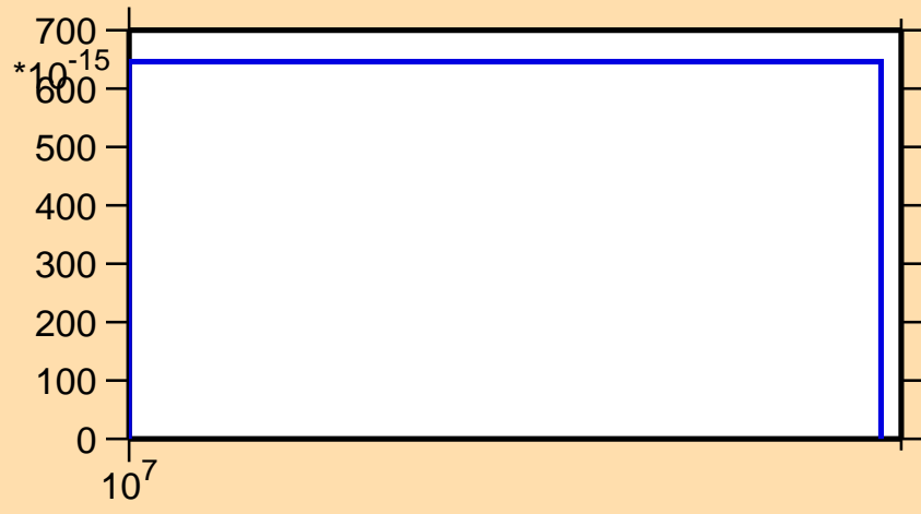
\sigma vs. E for ^{65}\text{Ga} (mt 34)
