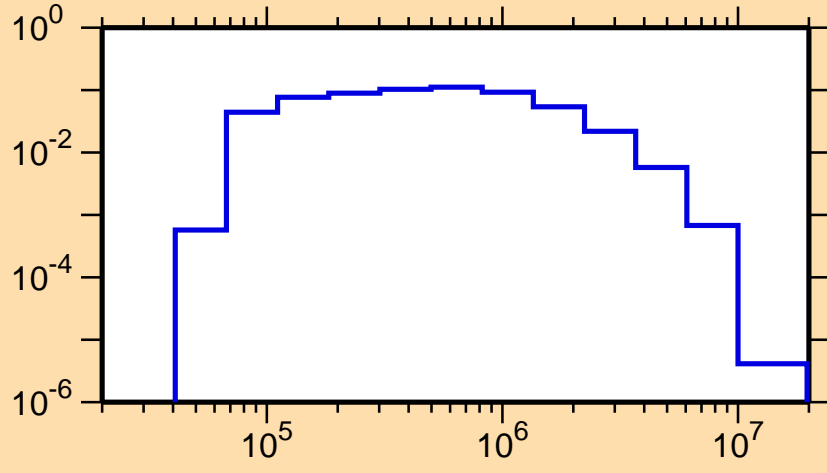
\sigma vs. E for ^{65}\text{Ga}(n,n_1)
