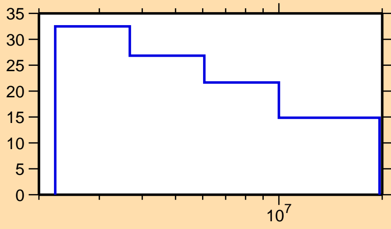
\Delta\sigma/\sigma vs. E for ^{65}\text{Ga}(n,n\text{cont.})
