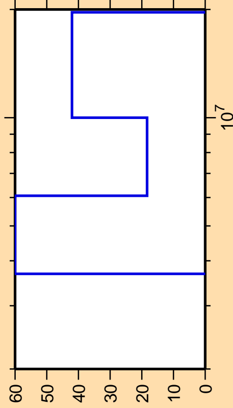
\Delta\sigma/\sigma vs. E for ^{65}\text{Ga}(n,n\alpha)
