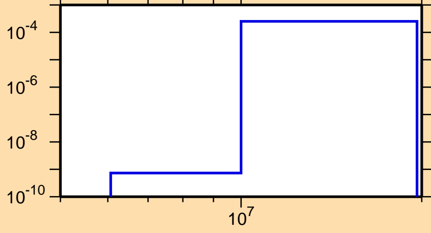
\sigma vs. E for ^{65}\text{Ga}(n,t)
