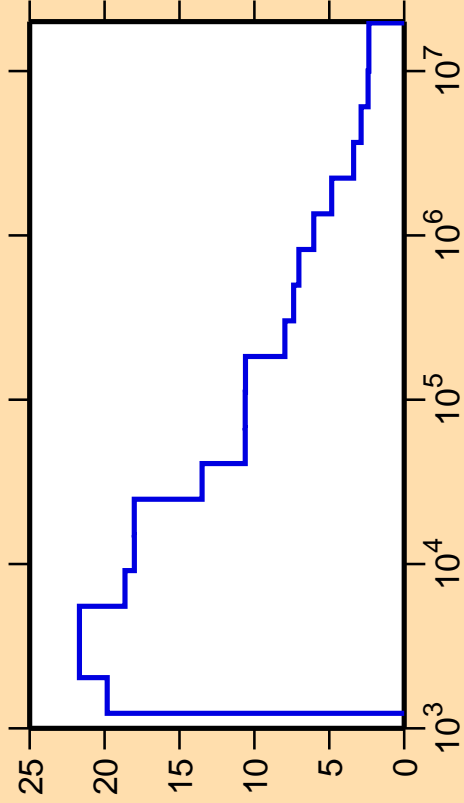
\Delta\sigma/\sigma vs. E for ^{65}\text{Ga}(n,\text{nonel.})
