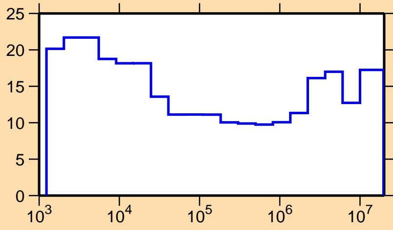
\Delta\sigma/\sigma vs. E for ^{65}\text{Ga}(n,p)
