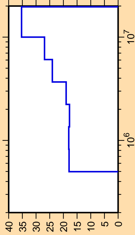
\Delta\sigma/\sigma vs. E for ^{65}\text{Ga}(n,n_3)
