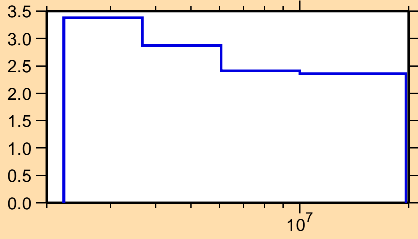
\Delta\sigma/\sigma vs. E for ^{65}\text{Ga}(n,n\text{nonel.})
