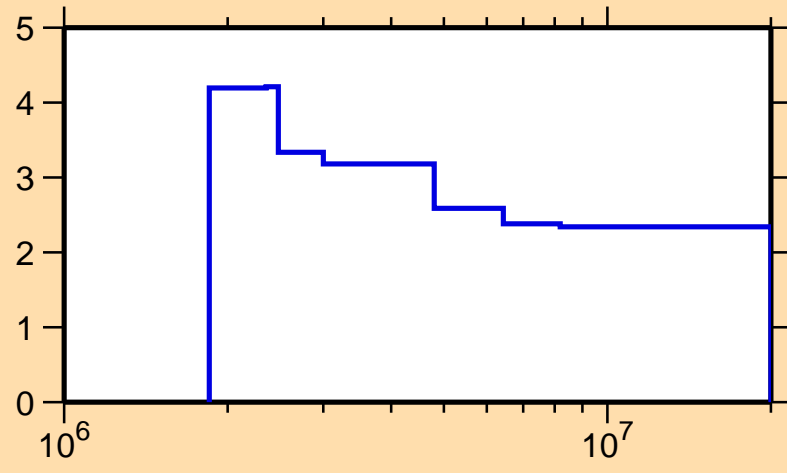
\Delta\sigma/\sigma vs. E for ^{65}\text{Ga}(n,n\text{nonel.})
