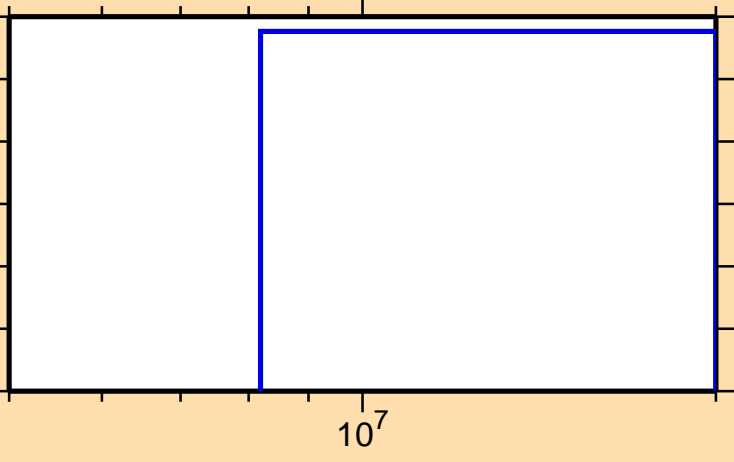
\sigma vs. E for ^{65}\text{Ga}(n,2n)
