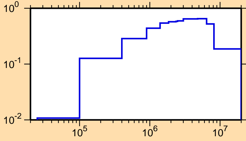
\sigma vs. E for ^{65}\text{Ga}(n,\text{inel.})
