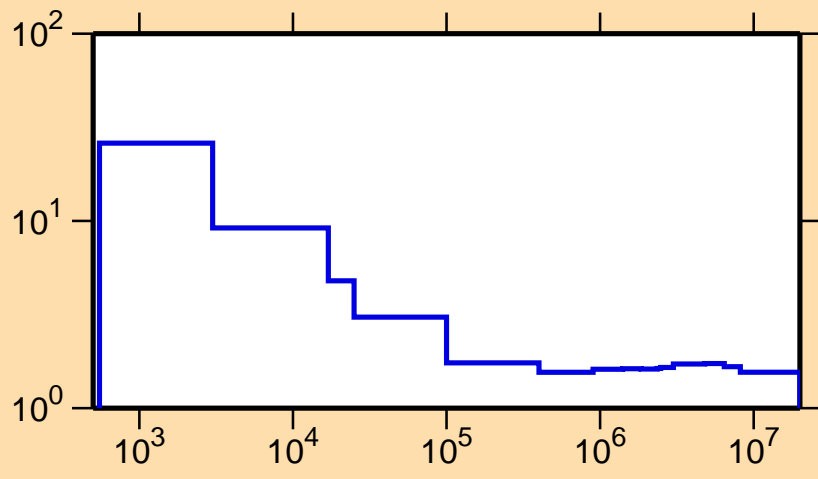
\sigma vs. E for ^{65}\text{Ga}(n,\text{nonel.})
