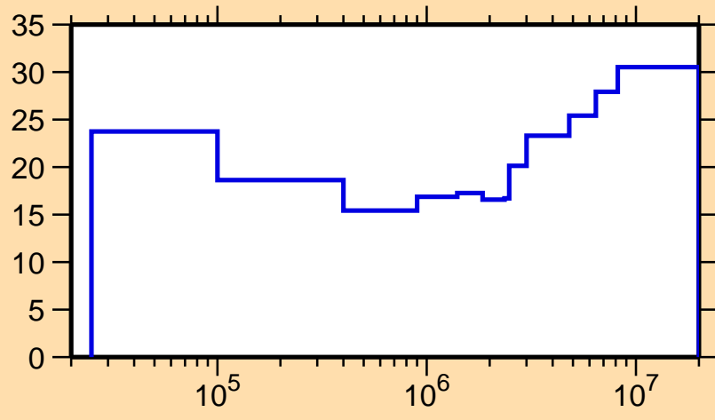
\Delta\sigma/\sigma vs. E for ^{65}\text{Ga}(n,n_1)
