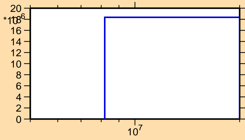
\sigma vs. E for ^{65}\text{Ga}(\text{mt117})
