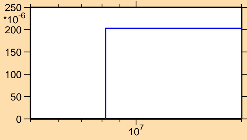
\sigma vs. E for ^{65}\text{Ga}(n,t)
