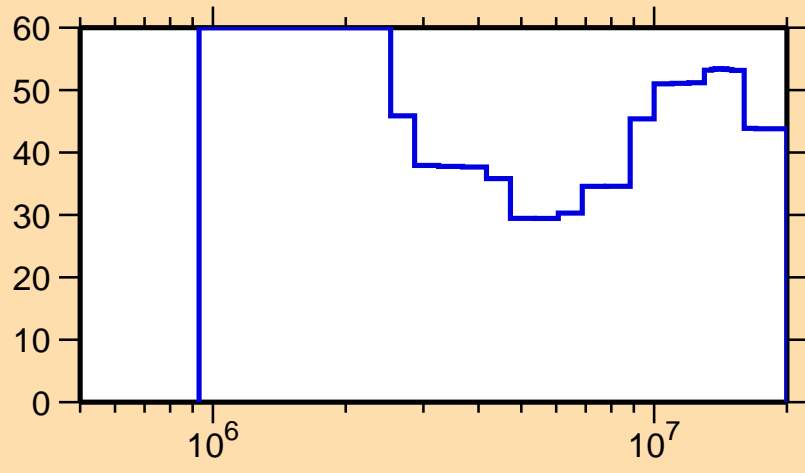
\Delta\sigma/\sigma vs. E for ^{66}\text{Ga}(n,ncont.)
