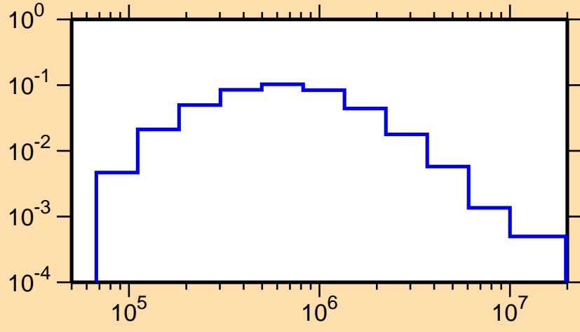
\sigma vs. E for ^{66}\text{Ga}(n,n_2)
