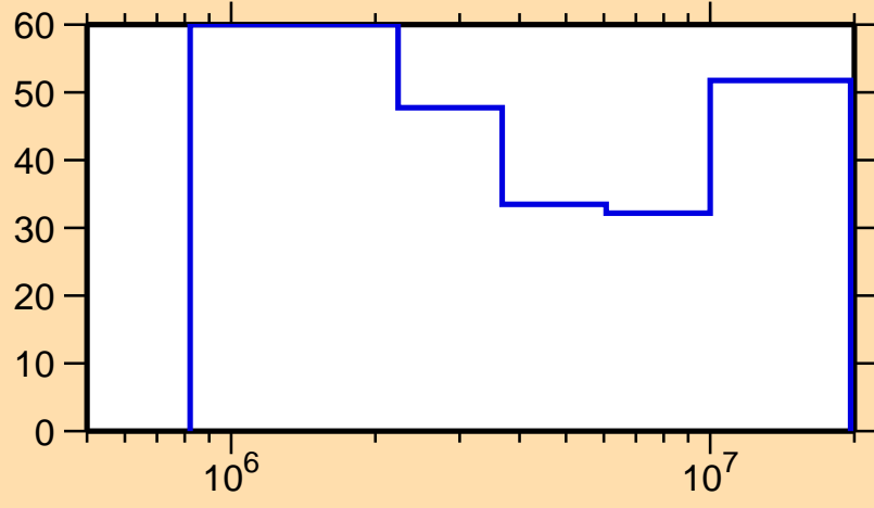
\Delta\sigma/\sigma vs. E for ^{66}\text{Ga}(n,ncont.)
