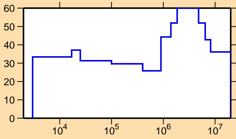
\Delta\sigma/\sigma vs. E for ^{66}\text{Ga}(n,p)
