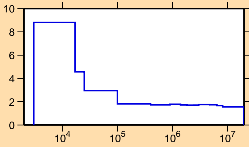
\sigma vs. E for ^{66}\text{Ga}(n,\text{nonel.})
