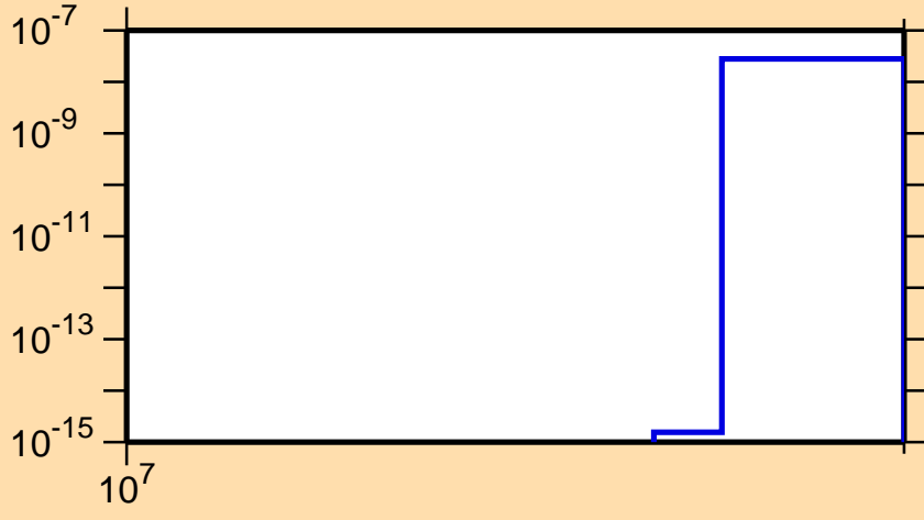
\sigma vs. E for ^{67}\text{Ga}(n,2n\alpha)
