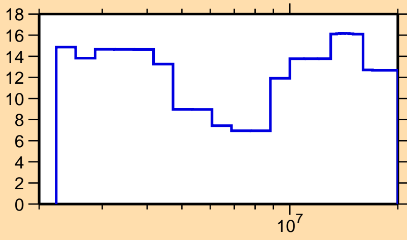
\Delta\sigma/\sigma vs. E for ^{67}\text{Ga}(n, el.)
