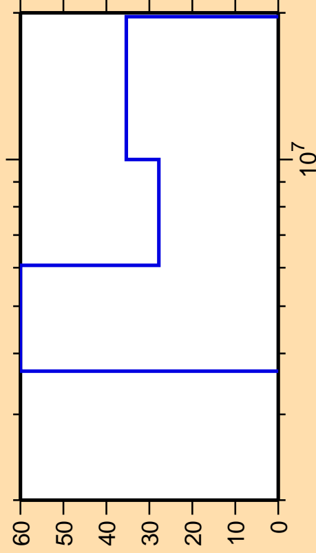
\Delta\sigma/\sigma vs. E for ^{67}\text{Ga}(n,np)
