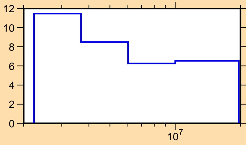
\Delta\sigma/\sigma vs. E for ^{67}\text{Ga}(n,n\text{inel.})
