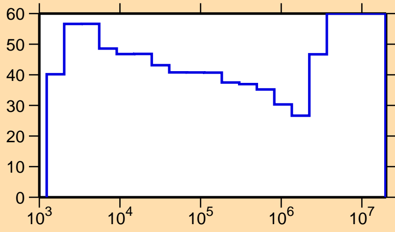
\Delta\sigma/\sigma vs. E for ^{67}\text{Ga}(n,p)
