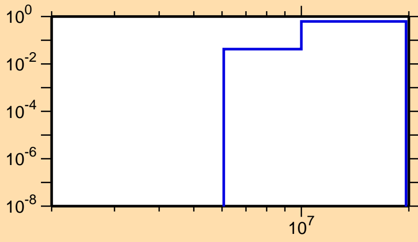
\sigma vs. E for ^{67}\text{Ga}(n,np)
