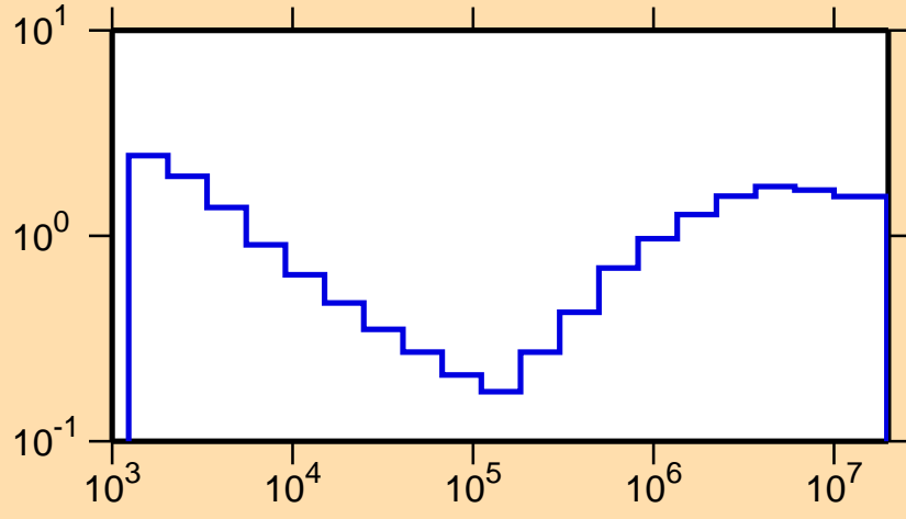
\sigma vs. E for ^{67}\text{Ga}(n,\text{nonel.})
