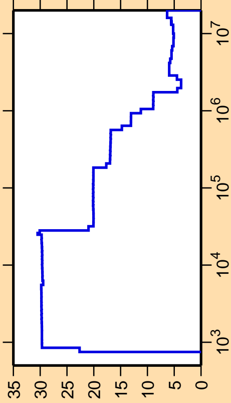
\Delta\sigma/\sigma vs. E for ^{68}\text{Ga}(n,\text{nonel.})
