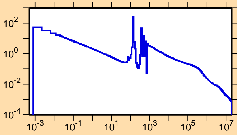
\sigma vs. E for ^{68}\text{Ga}(n,\gamma)
