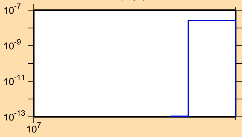
\sigma vs. E for ^{68}\text{Ga}(n,\text{pt})
