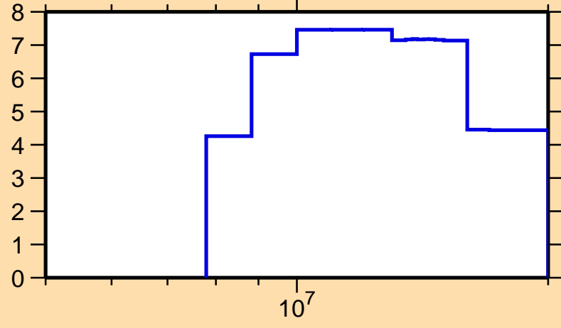
\Delta\sigma/\sigma vs. E for ^{68}\text{Ga}(n,\text{tot.})
