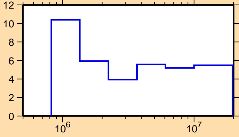
\Delta\sigma/\sigma vs. E for ^{68}\text{Ga}(n,n\text{nonel.})
