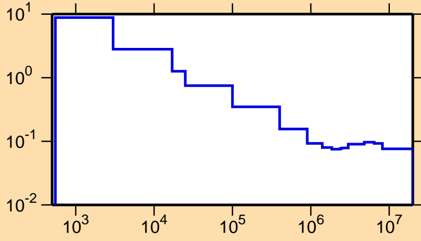
\sigma vs. E for ^{68}\text{Ga}(n,p)
