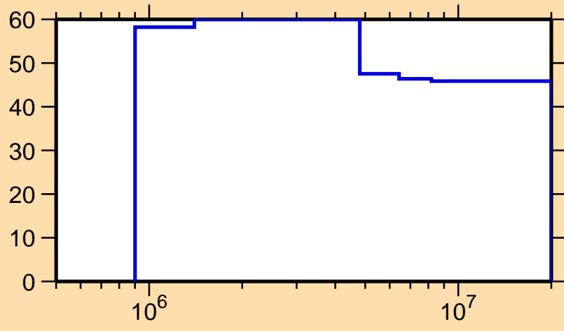
\Delta\sigma/\sigma vs. E for ^{68}\text{Ga}(n,n_1)
