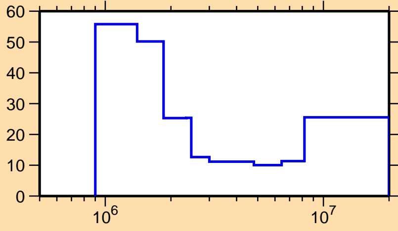
\Delta\sigma/\sigma vs. E for ^{68}\text{Ga}(n,n\text{cont.})
