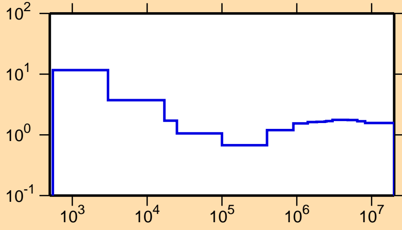
\sigma vs. E for ^{68}\text{Ga}(n,\text{nonel.})
