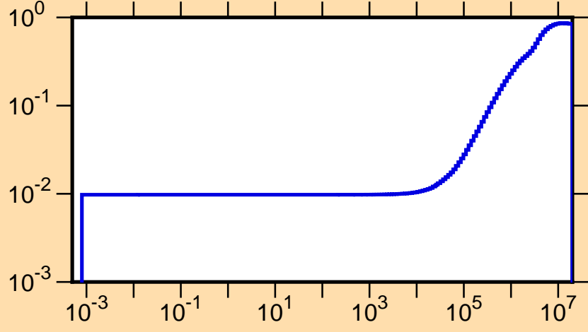
\mu vs. E for ^{69}\text{Ga}(\text{mt251})
