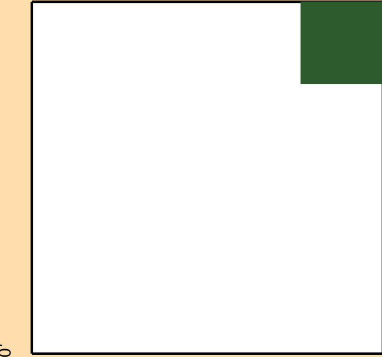
Correlation Matrix
