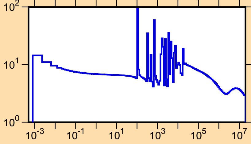
\sigma vs. E for ^{69}\text{Ga}(n,\text{tot.})
