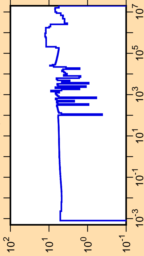
\Delta\sigma/\sigma vs. E for ^{69}\text{Ga}(n,\text{tot.})
