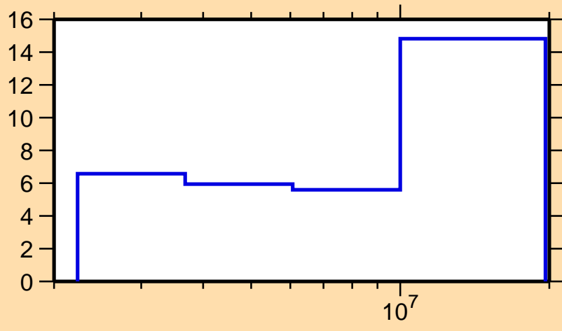
\Delta\sigma/\sigma vs. E for ^{69}\text{Ga}(n,ncont.)
