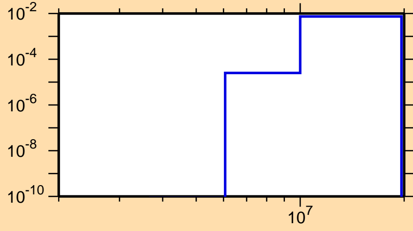
\sigma vs. E for ^{69}\text{Ga}(n,d)
