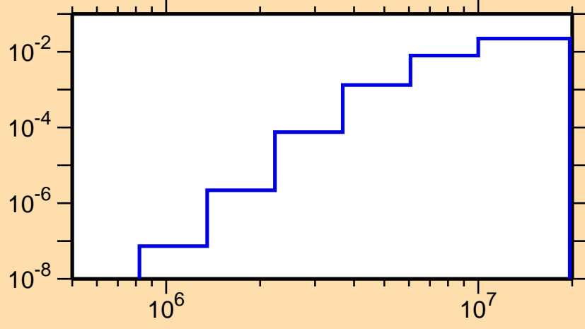
\sigma vs. E for ^{69}\text{Ga}(n,\alpha)
