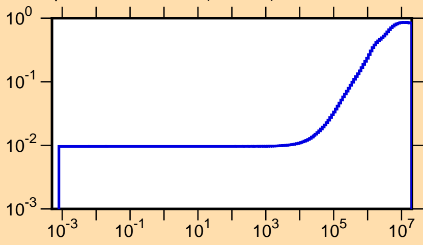
\mu vs. E for ^{70}\text{Ga}(\text{mt251})
