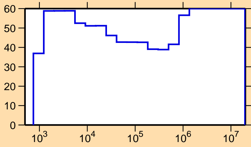
\Delta\sigma/\sigma vs. E for ^{70}\text{Ga}(n,p)
