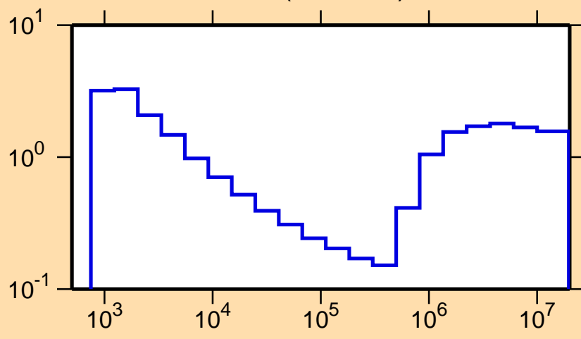
\sigma vs. E for ^{70}\text{Ga}(n,\text{nonel.})
