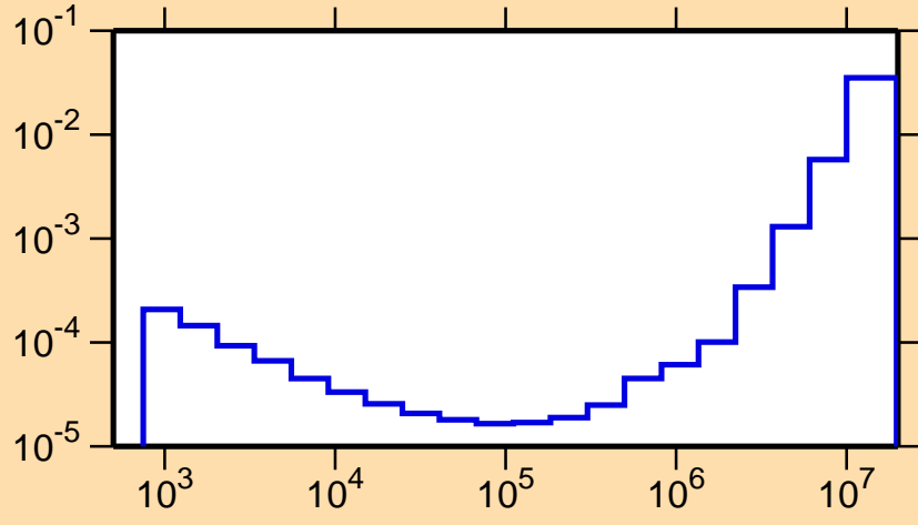
\sigma vs. E for ^{70}\text{Ga}(n,\alpha)
