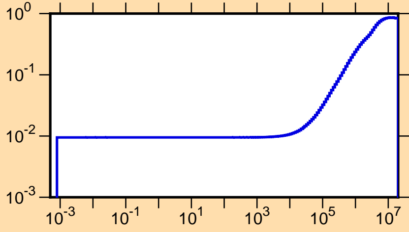
\mu vs. E for ^{71}\text{Ga}(\text{mt251})
