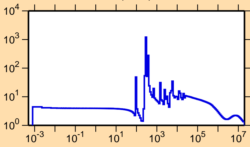
\sigma vs. E for ^{71}\text{Ga}(n,\text{el.})
