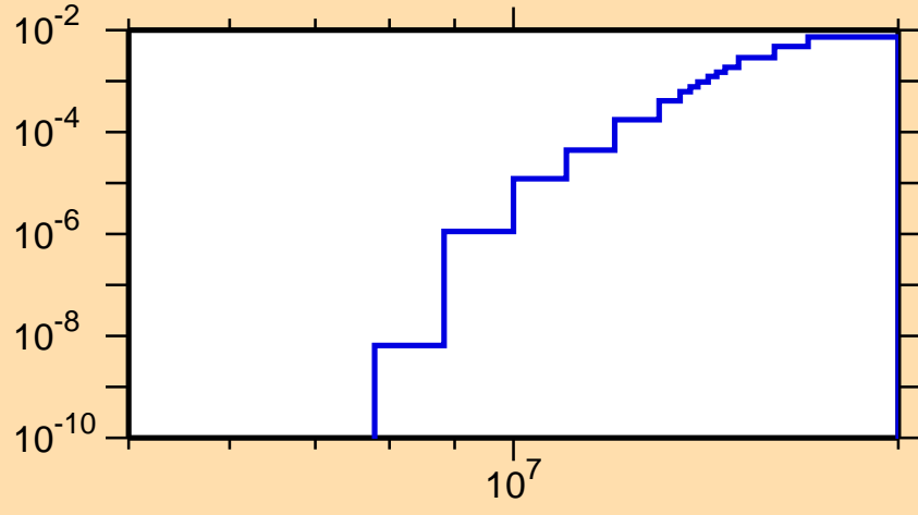
\sigma vs. E for ^{71}\text{Ga}(n,n\alpha)
