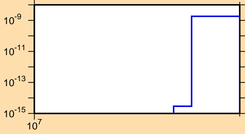
\sigma vs. E for ^{71}\text{Ga}(n,2n\alpha)
