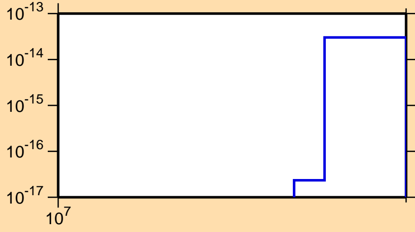
\sigma vs. E for ^{71}\text{Ga} (mt 45)
