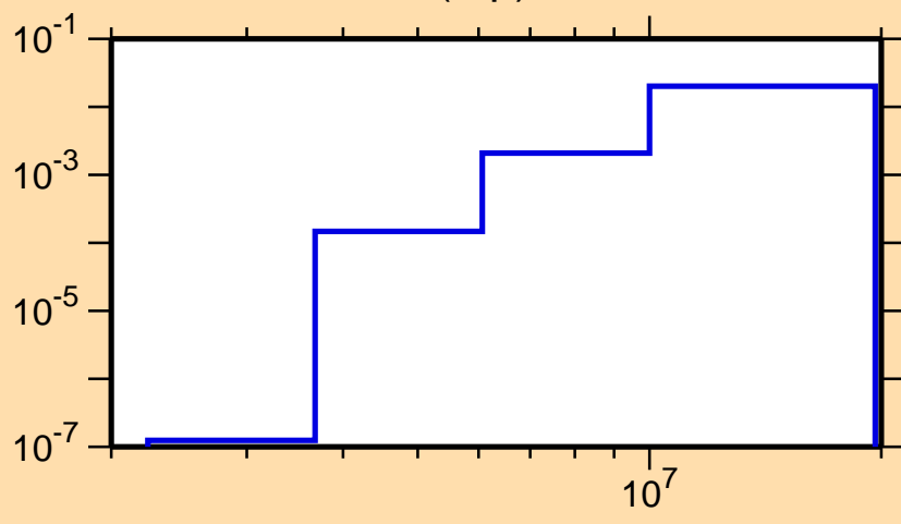
\sigma vs. E for ^{71}\text{Ga}(n,p)
