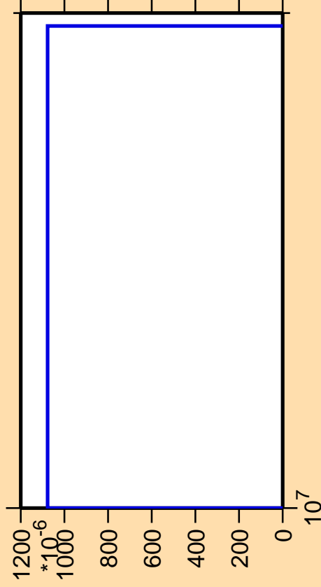
\Delta\sigma/\sigma vs. E for ^{71}\text{Ga} (mt 45)
