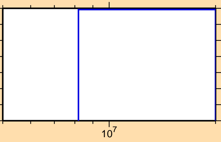
\sigma vs. E for ^{71}\text{Ga}(n,nt)
