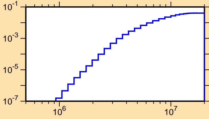
\sigma vs. E for ^{72}\text{Ga}(n,p)
