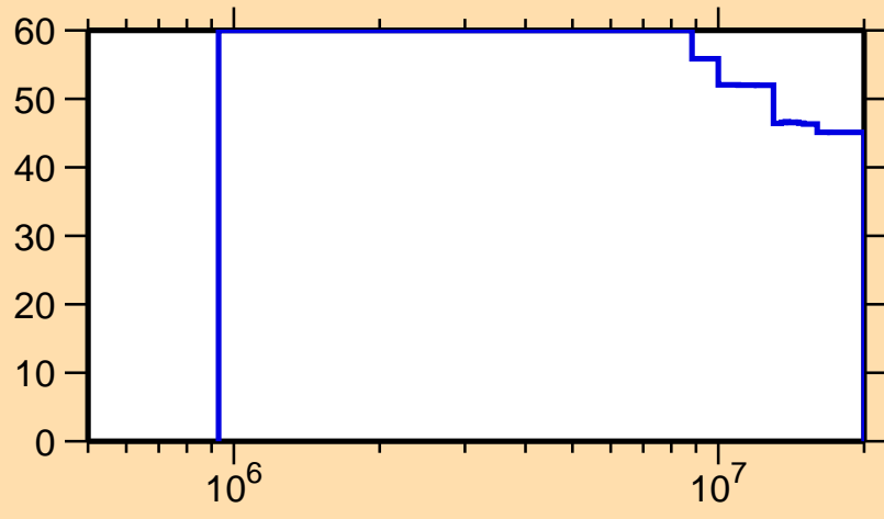
\Delta\sigma/\sigma vs. E for ^{72}\text{Ga}(n,p)
