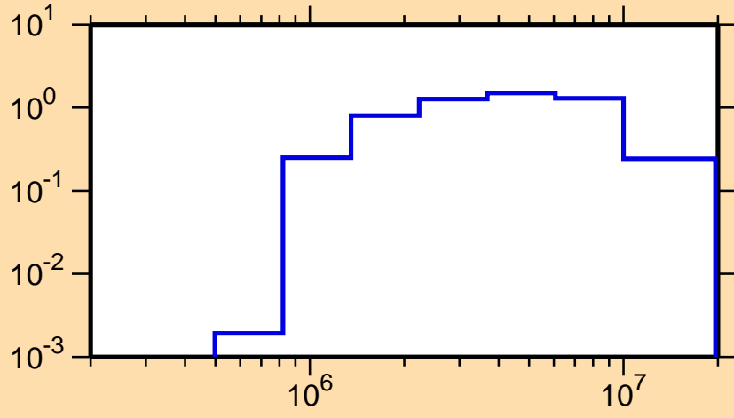
\sigma vs. E for ^{72}\text{Ga}(n,n\text{cont.})
