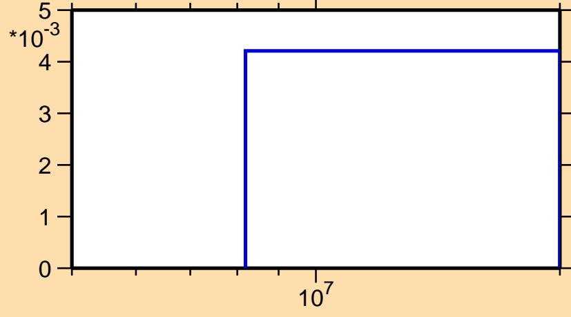
\sigma vs. E for ^{72}\text{Ga}(n,np)
