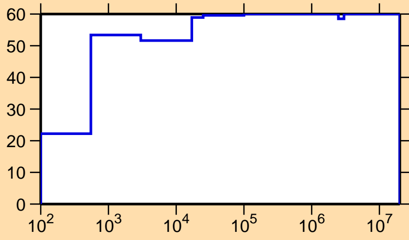
\Delta\sigma/\sigma vs. E for ^{72}\text{Ga}(n,\gamma)
