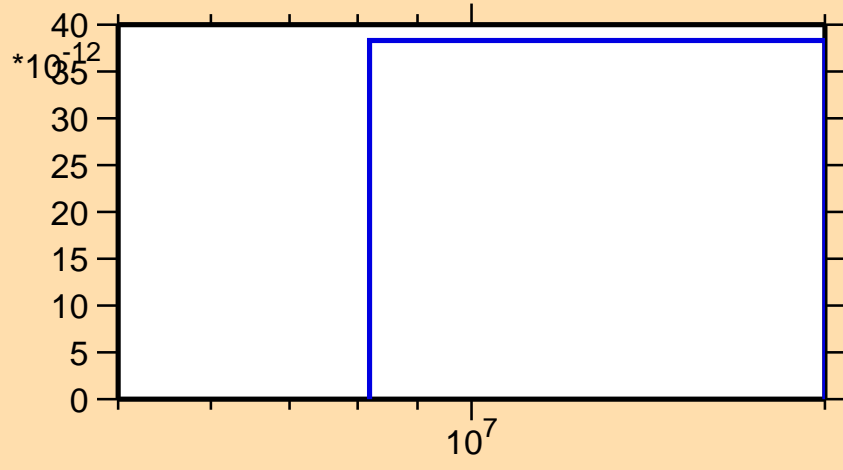
\sigma vs. E for ^{72}\text{Ga}(n,\text{He3})
