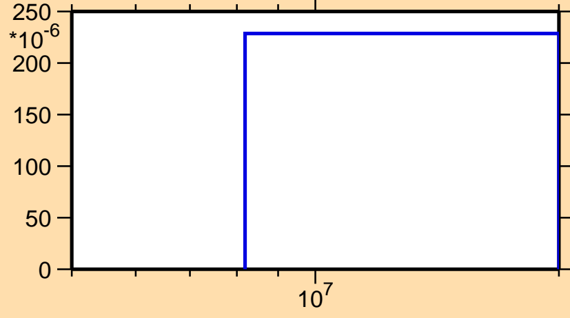
\sigma vs. E for ^{72}\text{Ga}(n,3n)
