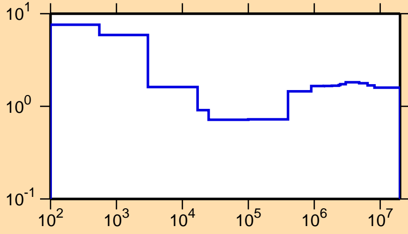
\sigma vs. E for ^{72}\text{Ga}(n,\text{nonel.})
