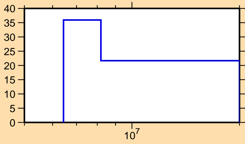
\Delta\sigma/\sigma vs. E for ^{72}\text{Ga}(n,2n)
