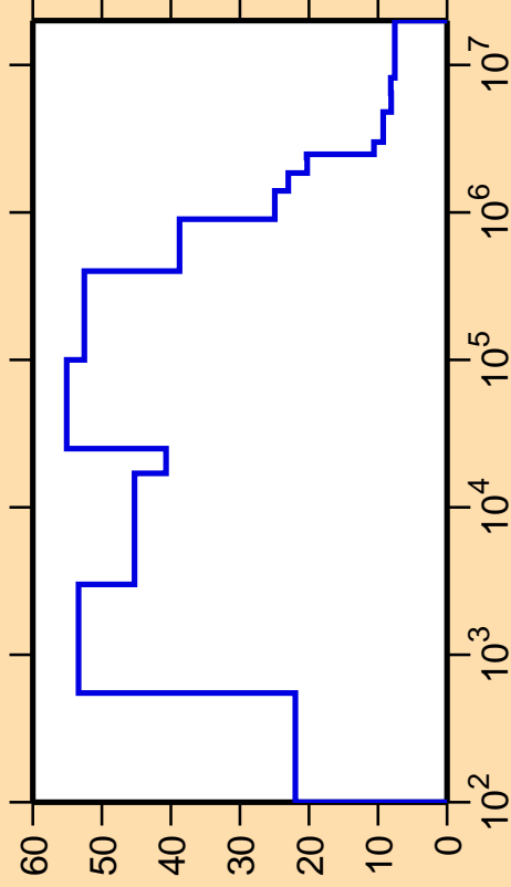
\Delta\sigma/\sigma vs. E for ^{72}\text{Ga}(n,\text{nonel.})
