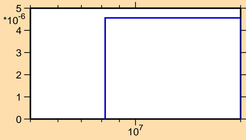
\sigma vs. E for ^{72}\text{Ga}(n,\text{nd})
