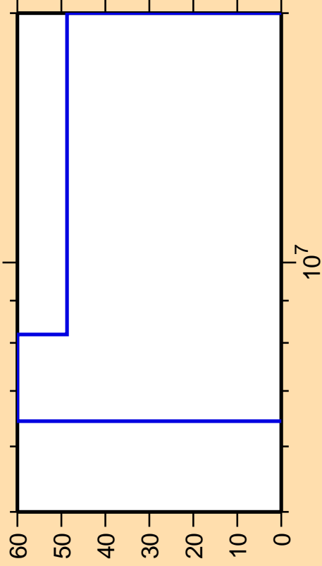
\Delta\sigma/\sigma vs. E for ^{72}\text{Ga}(n,p)
