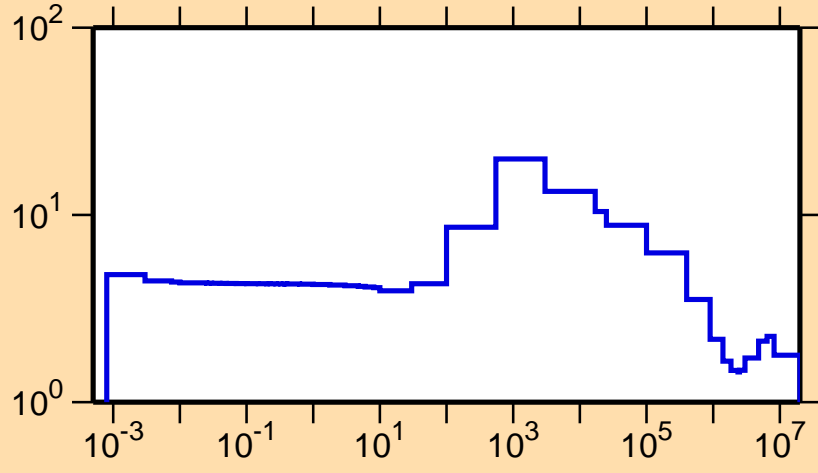
\sigma vs. E for ^{72}\text{Ga}(n,\text{el.})
