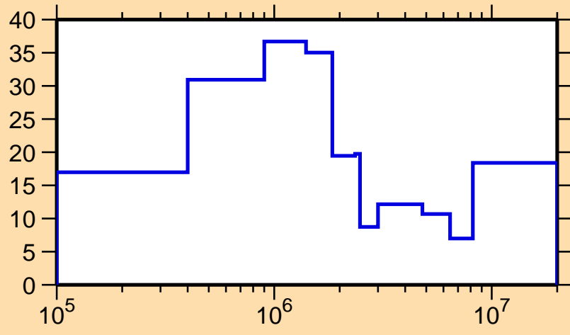
\Delta\sigma/\sigma vs. E for ^{72}\text{Ga}(n,el.)
