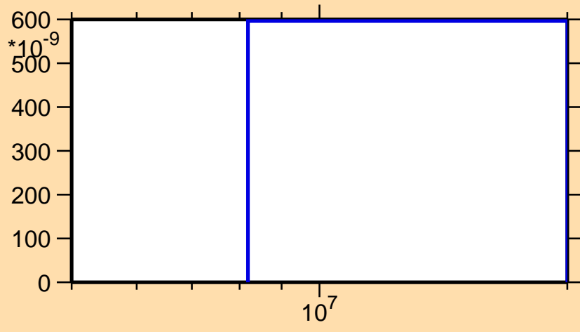
\sigma vs. E for ^{72}\text{Ga}(n,2np)
