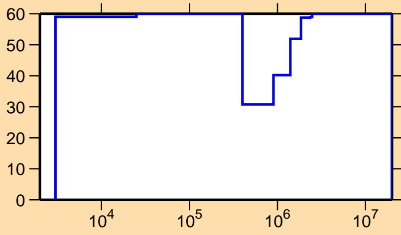
\Delta\sigma/\sigma vs. E for ^{72}\text{Ga}(n,n_1)
