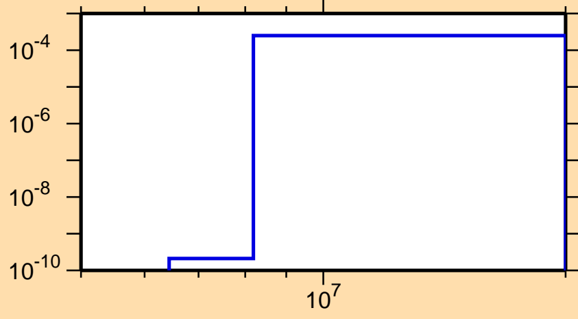
\sigma vs. E for ^{72}\text{Ga}(n,t)
