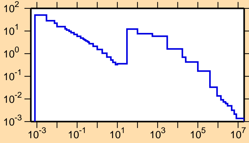
\sigma vs. E for ^{72}\text{Ga}(n,\gamma)
