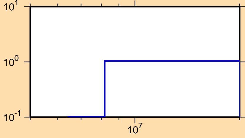
\sigma vs. E for ^{72}\text{Ga}(n,2n)
