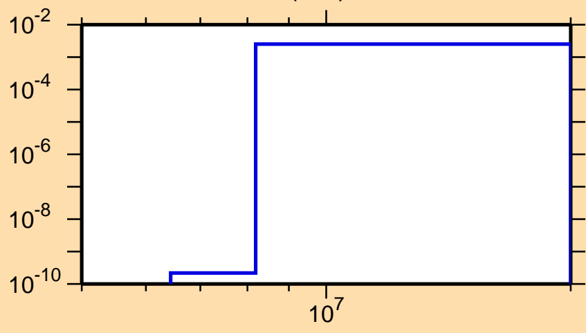
\sigma vs. E for ^{72}\text{Ga}(n,d)
