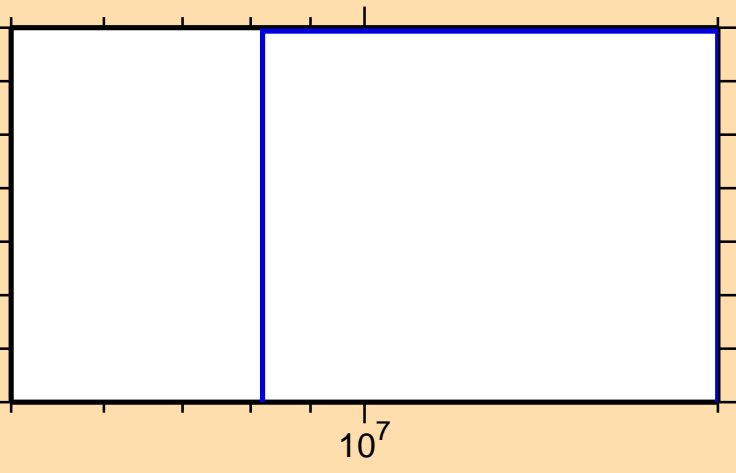
\sigma vs. E for ^{72}\text{Ga}(n,nt)
