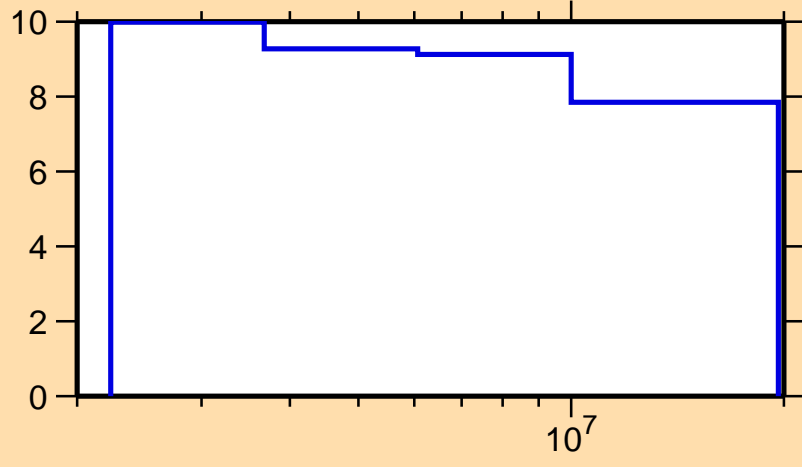
\Delta\sigma/\sigma vs. E for ^{73}\text{Ga}(n,n\text{nonel.})
