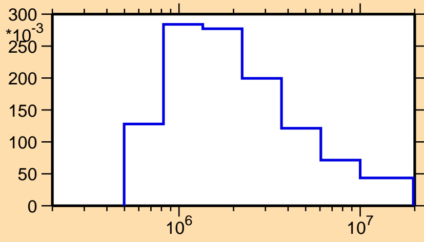
\sigma vs. E for ^{73}\text{Ga}(n,n_3)
