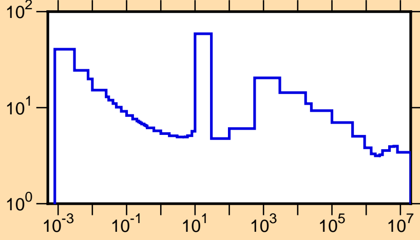
\sigma vs. E for ^{74}\text{Ga}(n,\text{tot.})
