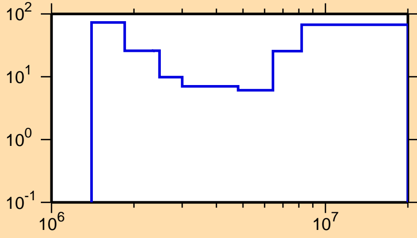
\Delta\sigma/\sigma vs. E for ^{74}\text{Ga}(n,n\text{cont.})
