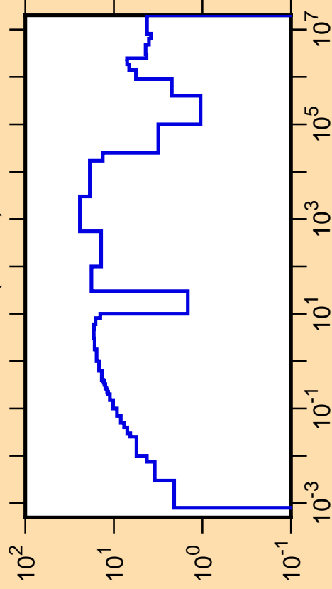
\Delta\sigma/\sigma vs. E for ^{74}\text{Ga}(n,\text{tot.})
