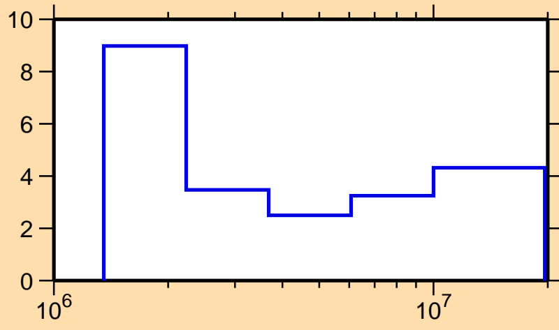
\Delta\sigma/\sigma vs. E for ^{74}\text{Ga}(n,n\text{onel.})
