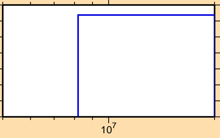
\sigma vs. E for ^{74}\text{Ga}(n,\text{He}3)
