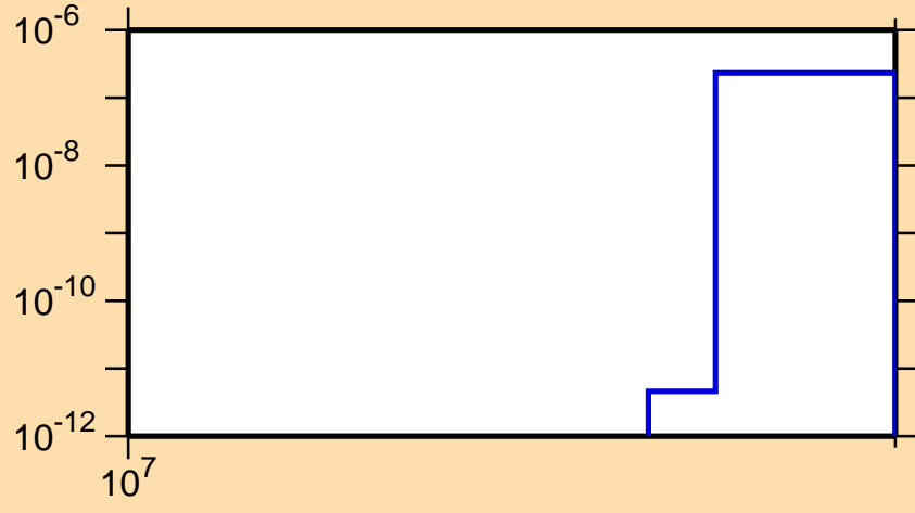
\sigma vs. E for ^{75}\text{Ga}(n,nt)
