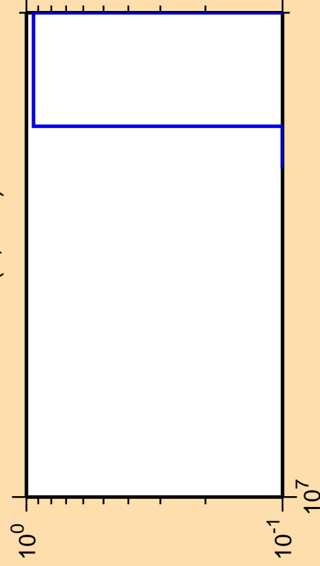
\Delta\sigma/\sigma vs. E for ^{75}\text{Ga}(n,2n\alpha)
