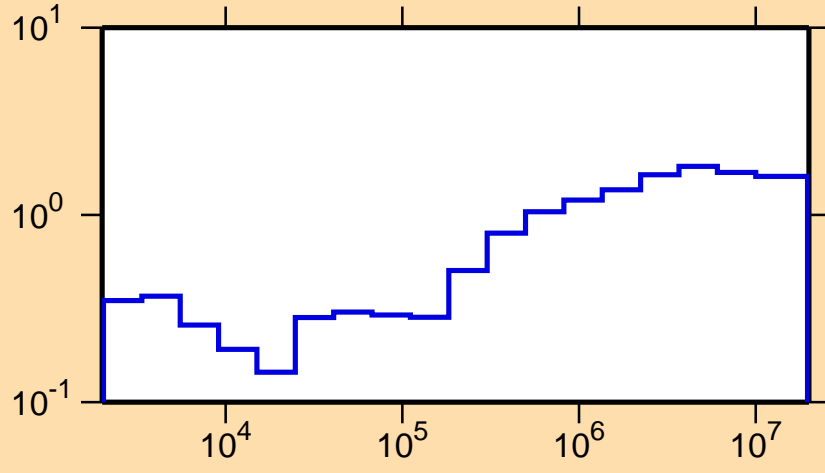
\sigma vs. E for ^{75}\text{Ga}(n,\text{nonel.})
