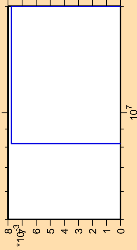
\Delta\sigma/\sigma vs. E for ^{75}\text{Ga}(n,2n\alpha)
