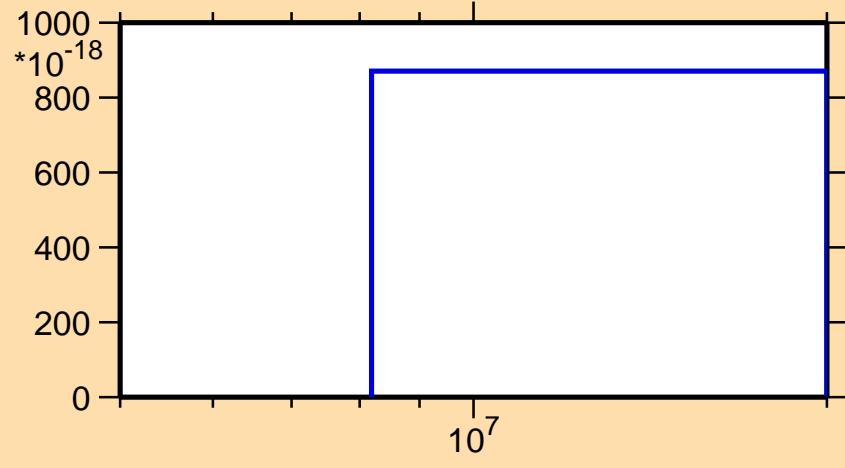
\sigma vs. E for ^{75}\text{Ga}(n,2n\alpha)
