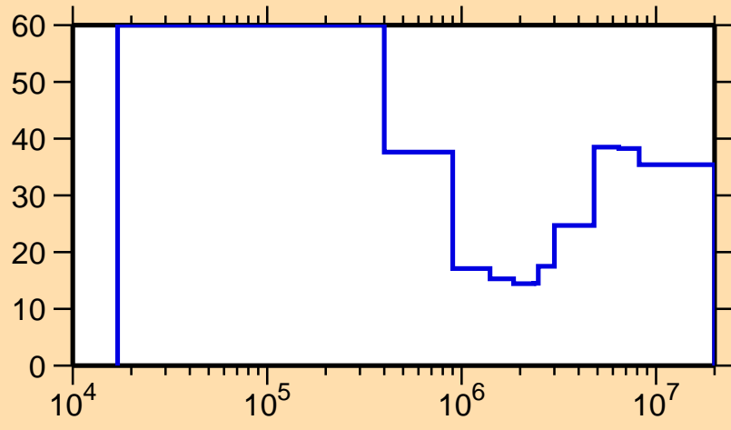
\Delta\sigma/\sigma vs. E for ^{75}\text{Ga}(n,n_1)
