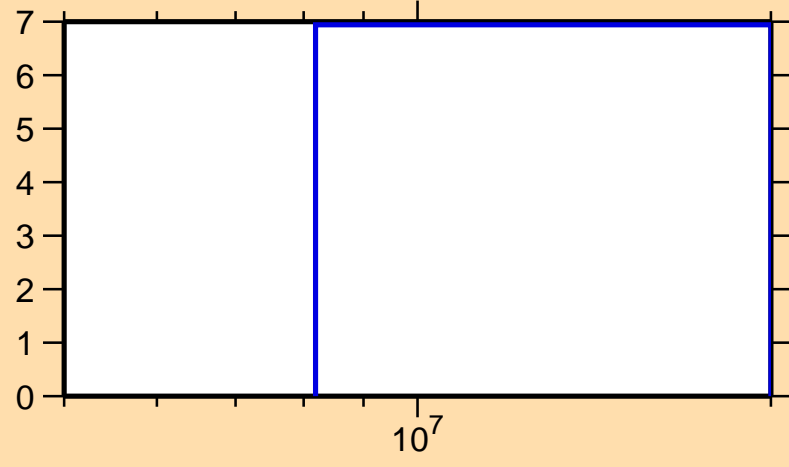
\Delta\sigma/\sigma vs. E for ^{75}\text{Ga}(n,\text{nonel.})
