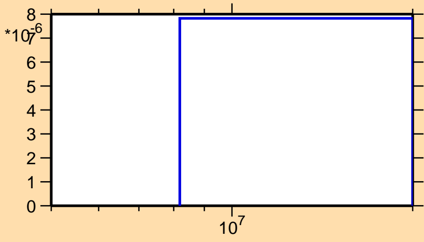
\sigma vs. E for ^{75}\text{Ga}(n,n\alpha)
