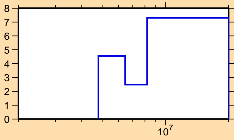
\Delta\sigma/\sigma vs. E for ^{75}\text{Ga}(n,\text{tot.})
