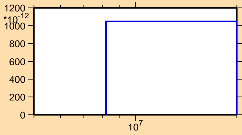
\sigma vs. E for ^{75}\text{Ga}(n,\text{nd})
