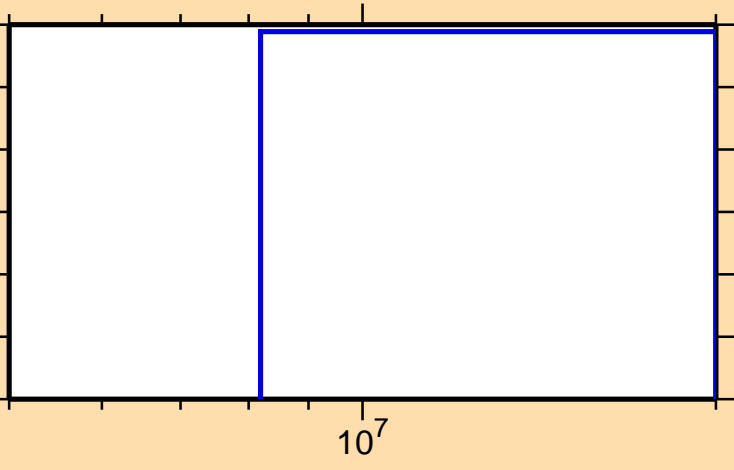
\sigma vs. E for ^{75}\text{Ga}(n,t)
