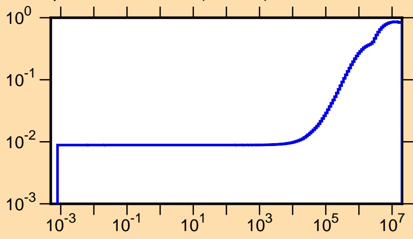
\mu vs. E for ^{76}\text{Ga}(\text{mt251})
