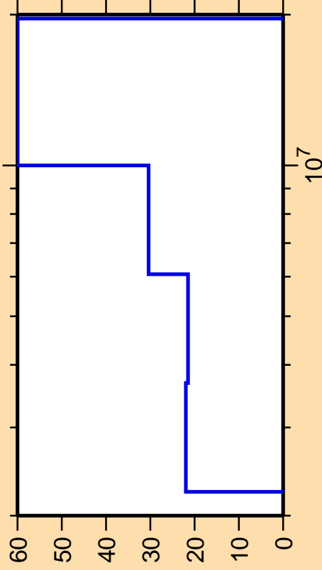
\Delta\sigma/\sigma vs. E for ^{76}\text{Ga}(n,\text{ncont.})
