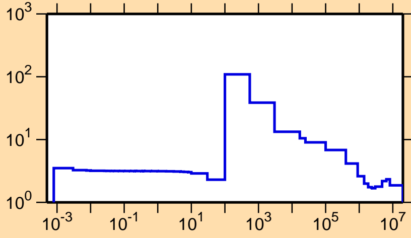
\sigma vs. E for ^{76}\text{Ga}(n,\text{el.})
