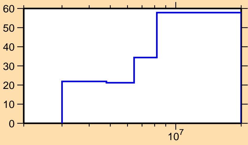
\Delta\sigma/\sigma vs. E for ^{76}\text{Ga}(n,ncont.)
