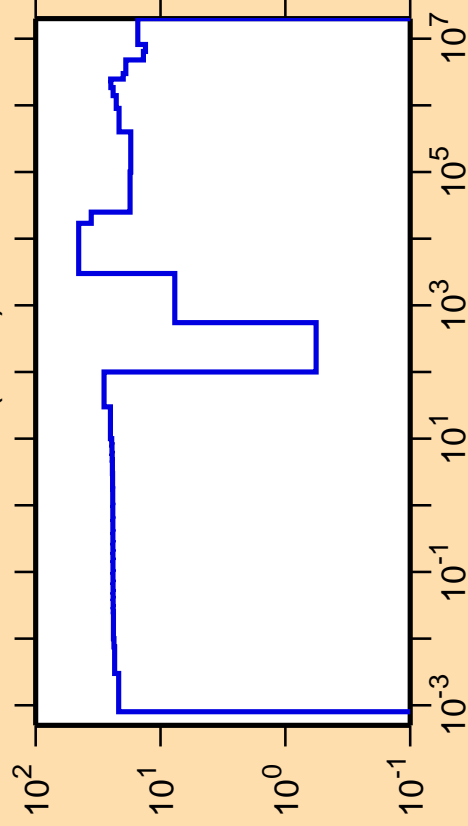
\Delta\sigma/\sigma vs. E for ^{76}\text{Ga}(n,\text{el.})
