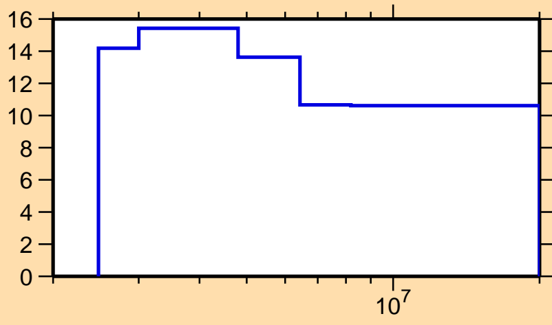
\Delta\sigma/\sigma vs. E for ^{76}\text{Ga}(n,n\text{nonel.})
