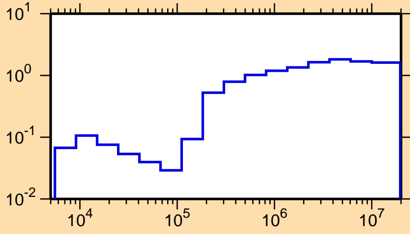
\sigma vs. E for ^{77}\text{Ga}(n,\text{nonel.})
