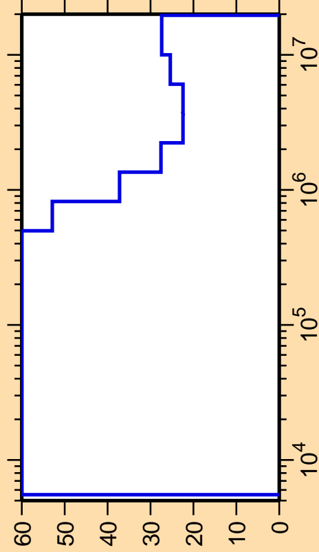
\Delta\sigma/\sigma vs. E for ^{77}\text{Ga}(n,\text{nonel.})
