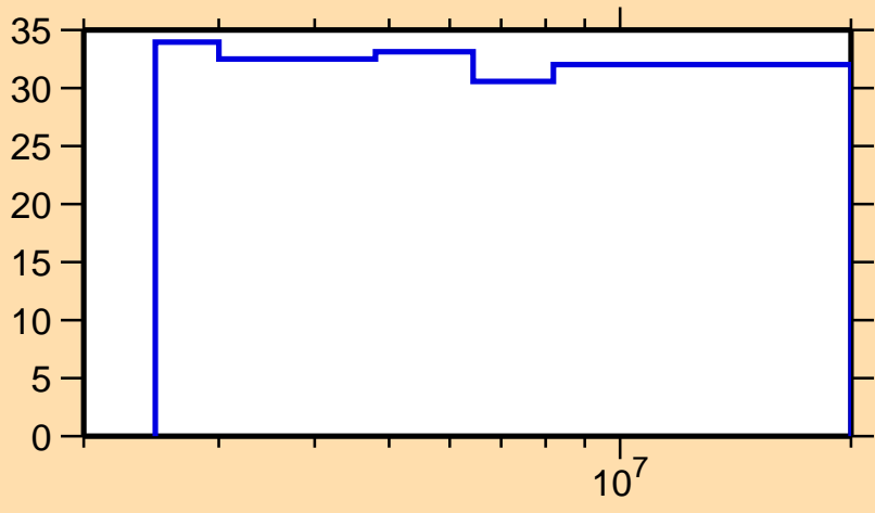
\Delta\sigma/\sigma vs. E for ^{77}\text{Ga}(n,n\text{cont.})
