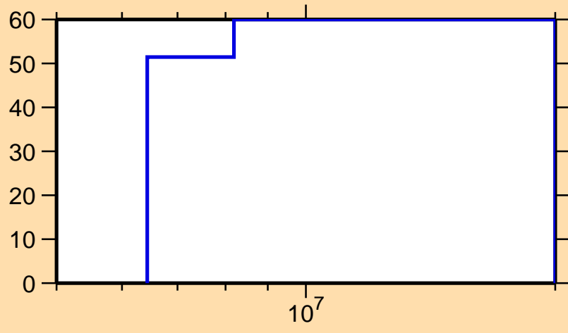
\Delta\sigma/\sigma vs. E for ^{77}\text{Ga}(n,\gamma)
