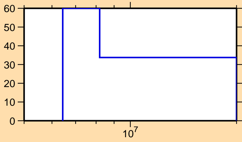
\Delta\sigma/\sigma vs. E for ^{77}\text{Ga}(n,2n)
