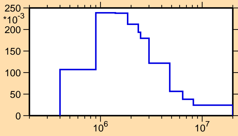
\sigma vs. E for ^{77}\text{Ga}(n,n_4)
