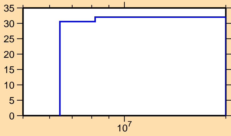
\Delta\sigma/\sigma vs. E for ^{77}\text{Ga}(n,ncont.)
