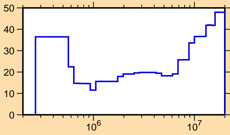
\Delta\sigma/\sigma vs. E for ^{78}\text{Ga}(n,\text{inel.})
