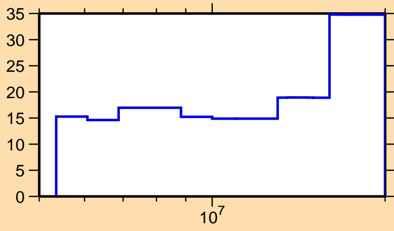
\Delta\sigma/\sigma vs. E for ^{78}\text{Ga}(n,2n)
