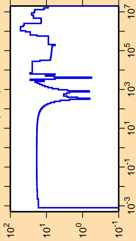
\Delta\sigma/\sigma vs. E for ^{78}\text{Ga}(n,\text{el.})
