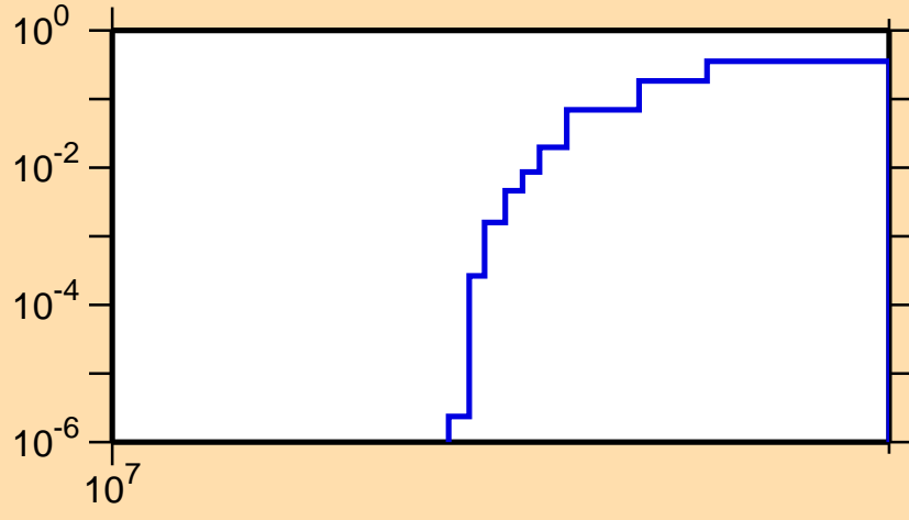
\sigma vs. E for ^{78}\text{Ga}(n,3n)
