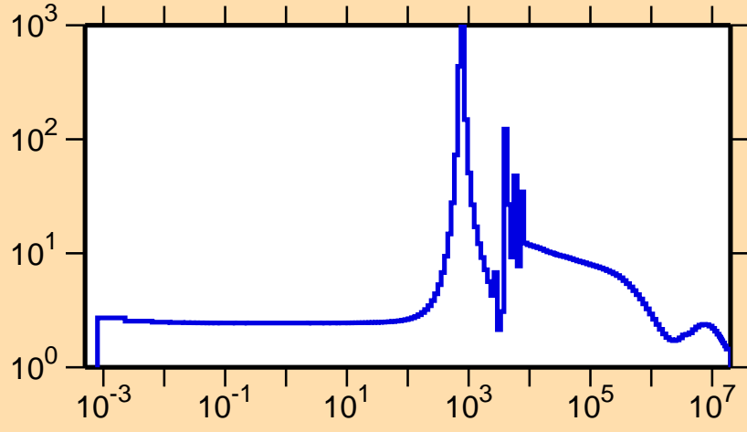
\sigma vs. E for ^{78}\text{Ga}(n,\text{el.})
