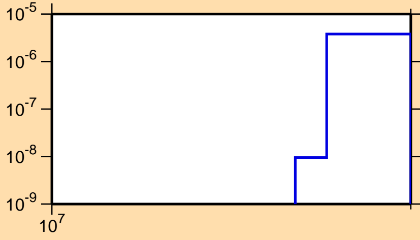
\sigma vs. E for ^{78}\text{Ga}(n,\text{nd})
