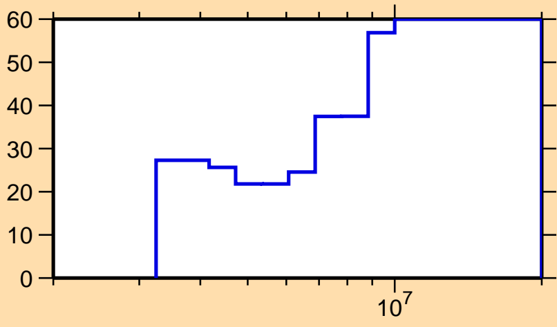
\Delta\sigma/\sigma vs. E for ^{78}\text{Ga}(n,n\text{cont.})
