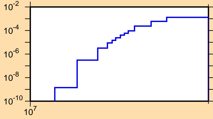
\sigma vs. E for ^{78}\text{Ga}(n,d)
