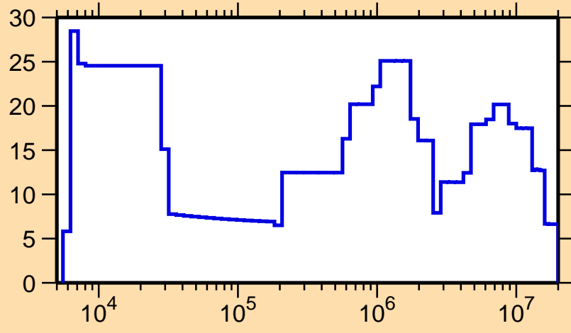
\Delta\sigma/\sigma vs. E for ^{78}\text{Ga}(n,\text{tot.})
