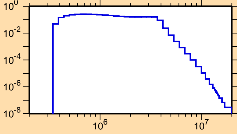
\sigma vs. E for ^{78}\text{Ga}(n,n_2)
