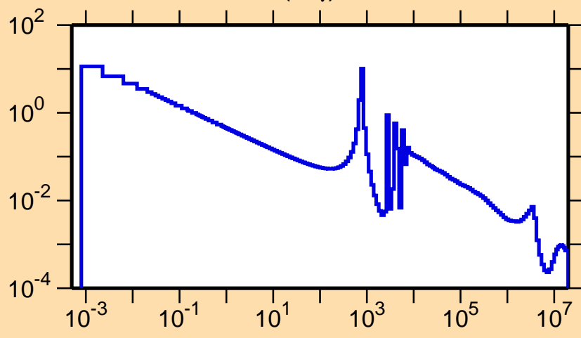
\sigma vs. E for ^{78}\text{Ga}(n,\gamma)
