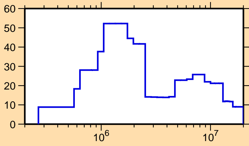
\Delta\sigma/\sigma vs. E for ^{78}\text{Ga}(n,\text{el.})
