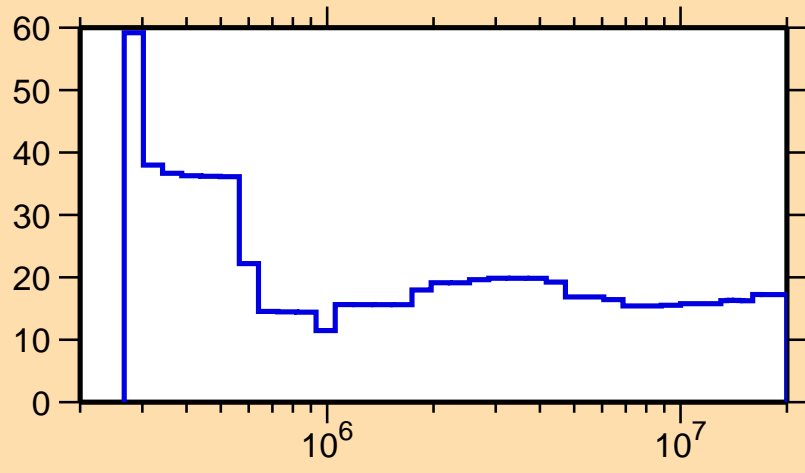
\Delta\sigma/\sigma vs. E for ^{78}\text{Ga}(n,\text{nonel.})
