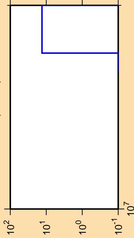
\Delta\sigma/\sigma vs. E for ^{78}\text{Ga}(n,2n\alpha)
