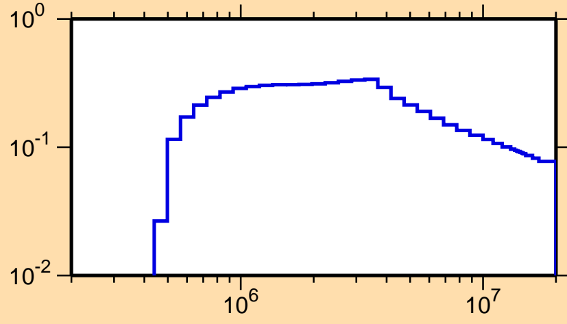
\sigma vs. E for ^{78}\text{Ga}(n,n_3)
