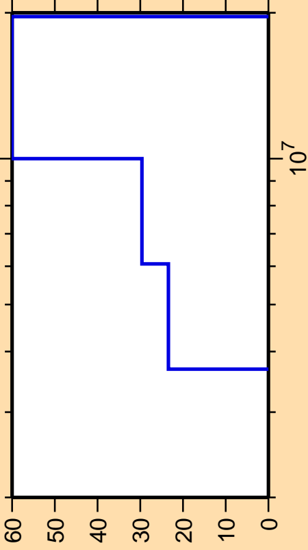
\Delta\sigma/\sigma vs. E for ^{78}\text{Ga}(n,n\text{cont.})
