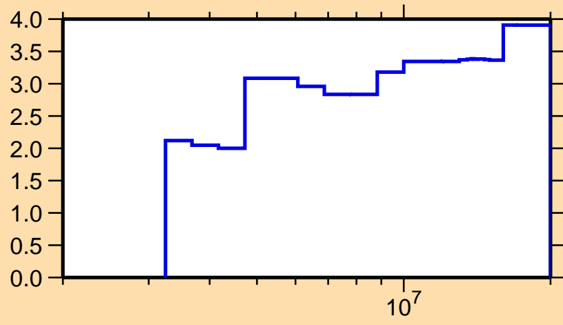
\Delta\sigma/\sigma vs. E for ^{79}\text{Ga}(n,n\text{inel.})
