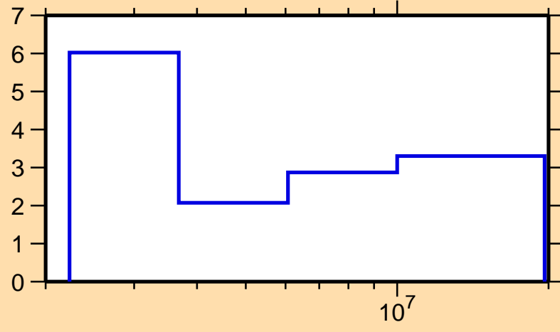
\Delta\sigma/\sigma vs. E for ^{79}\text{Ga}(n,n\text{inel.})
