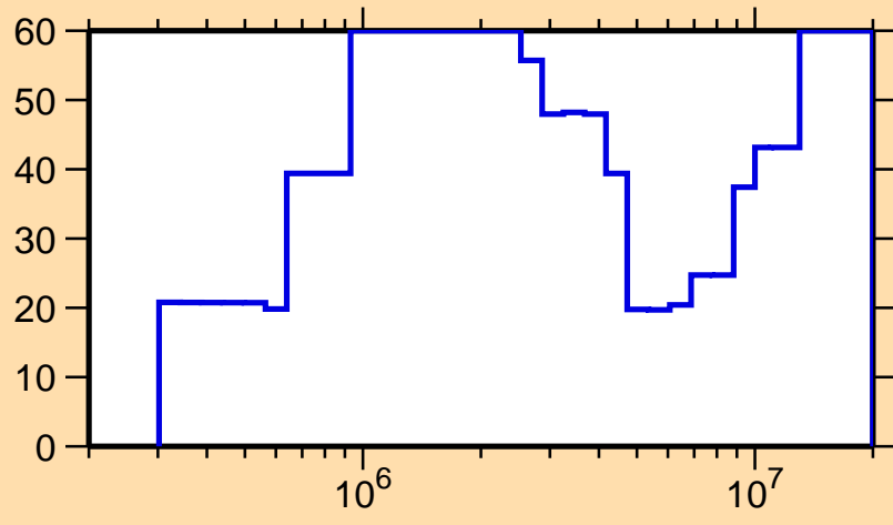
\Delta\sigma/\sigma vs. E for ^{80}\text{Ga}(n,\text{el.})
