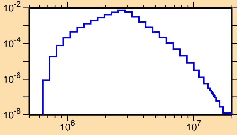
\sigma vs. E for ^{80}\text{Ga}(n,n_4)
