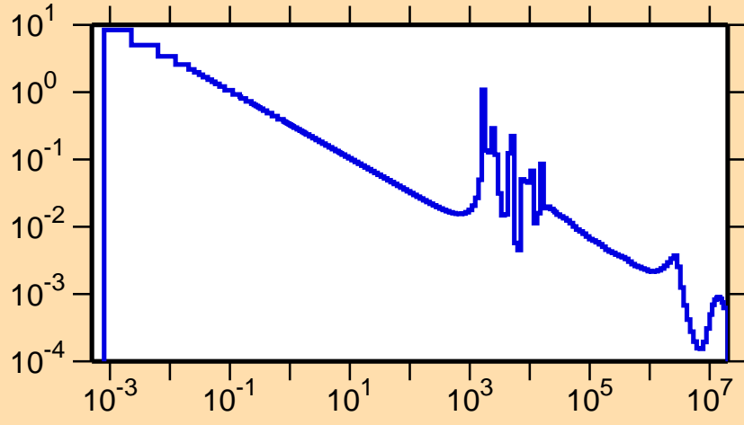
\sigma vs. E for ^{80}\text{Ga}(n,\gamma)
