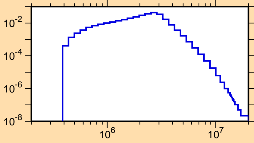
\sigma vs. E for ^{80}\text{Ga}(n,n_2)
