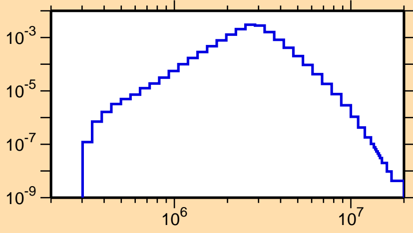
\sigma vs. E for ^{80}\text{Ga}(n,n_1)
