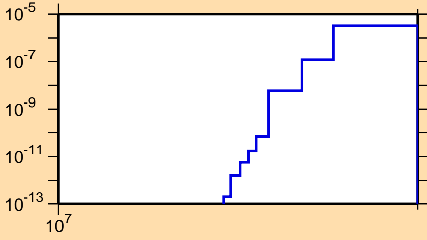
\sigma vs. E for ^{80}\text{Ga}(n,n\alpha)
