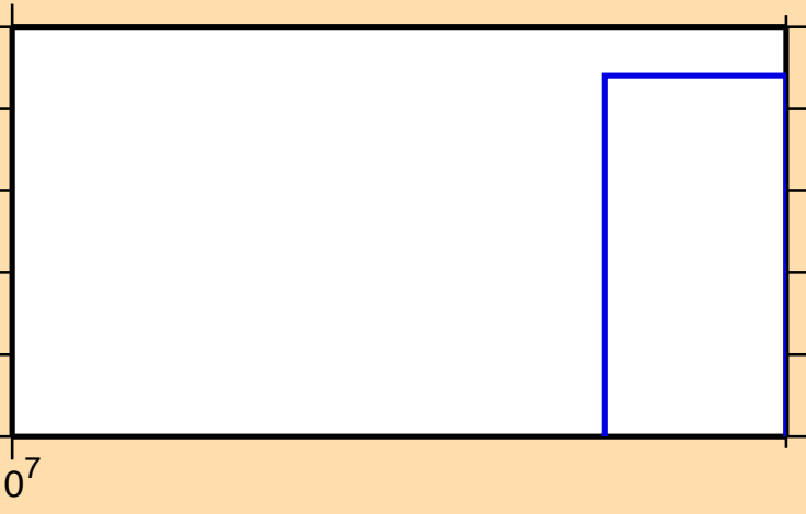
\sigma vs. E for ^{80}\text{Ga}(n,2np)
