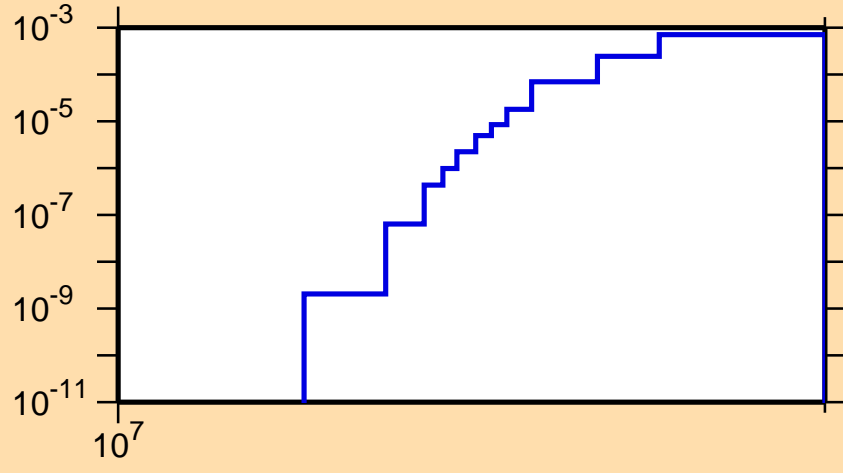
\sigma vs. E for ^{80}\text{Ga}(n,d)
