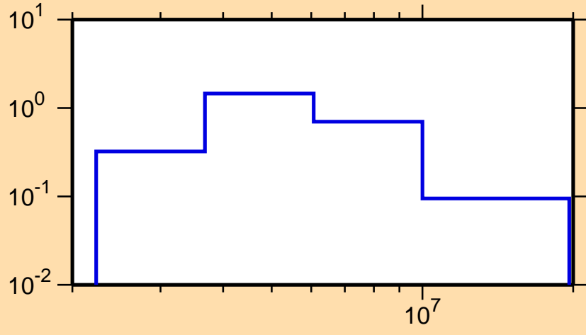
\sigma vs. E for ^{80}\text{Ga}(n,n\text{cont.})
