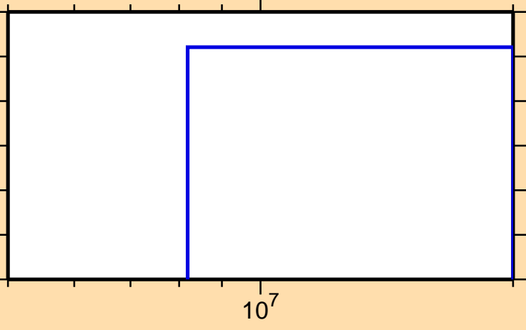
\sigma vs. E for ^{80}\text{Ga}(n,d)
