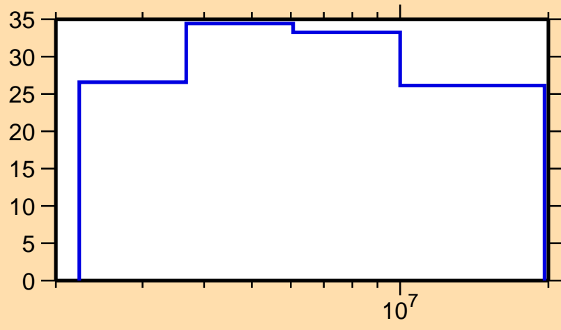
\Delta\sigma/\sigma vs. E for ^{81}\text{Ga}(n,n\text{nonel.})
