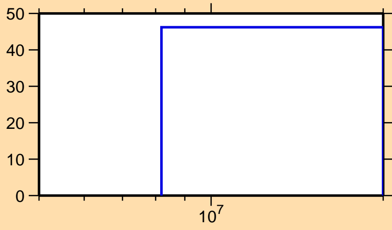
\Delta\sigma/\sigma vs. E for ^{81}\text{Ga}(n,el.)
