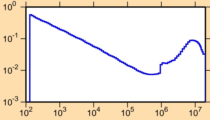
\sigma vs. E for ^{135}\text{Gd}(n,\alpha)
