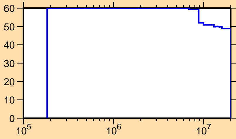
\Delta\sigma/\sigma vs. E for ^{135}\text{Gd}(n,ncont.)
