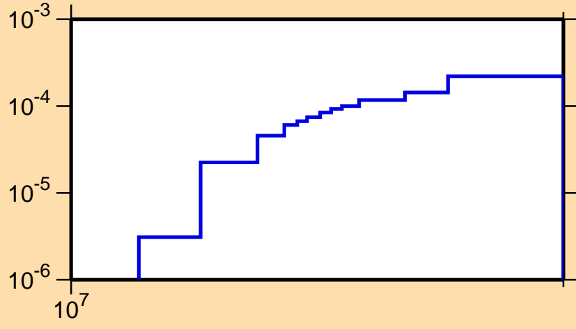
\sigma vs. E for ^{135}\text{Gd}(n,2n)
